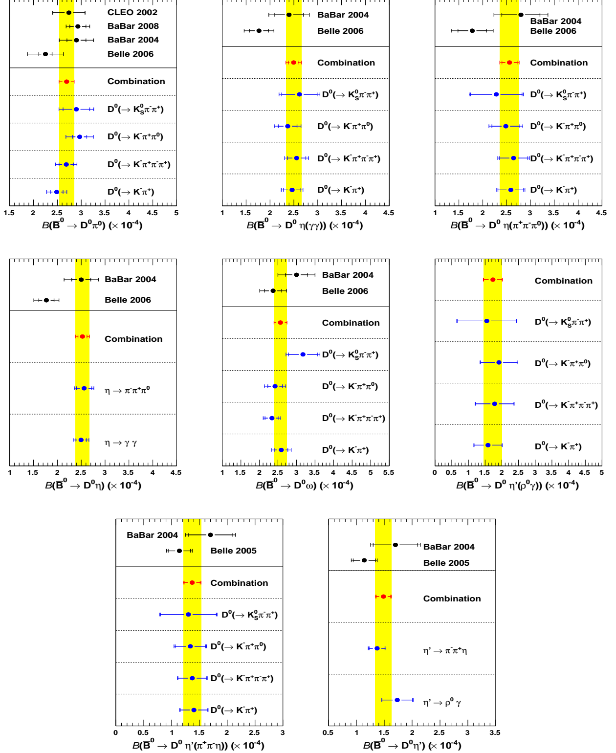
FIG. 5: \mathcal{B}(\bar{B}^0 \rightarrow D^0 h^0) (\times 10^{-4}) for the individual reconstructed D^0 and h^0 decay channels (blue points) together with the BLUE combination of this paper measurements (vertical yellow bands and the red points). The previous experimental results from BABAR [7, 14], Belle [11, 12], and CLEO [10] are also shown (black points). The horizontal bars represent the statistical contribution alone and the quadratic sum of the statistical and systematic uncertainty contributions. The width of the vertical yellow band corresponds to \pm 1\sigma of the combined measurement, where the statistical and systematic uncertainties are summed in quadrature.
