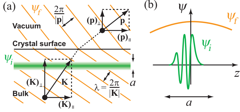
FIG. 3: (Color online) Photoemission from a 2D state into an inverse LEED state. (a) A schematic of the 2D and inverse LEED states. Orange lines show wave fronts that are refracted at the surface. (b) A schematic of the wave functions of the 2D and inverse LEED states.
