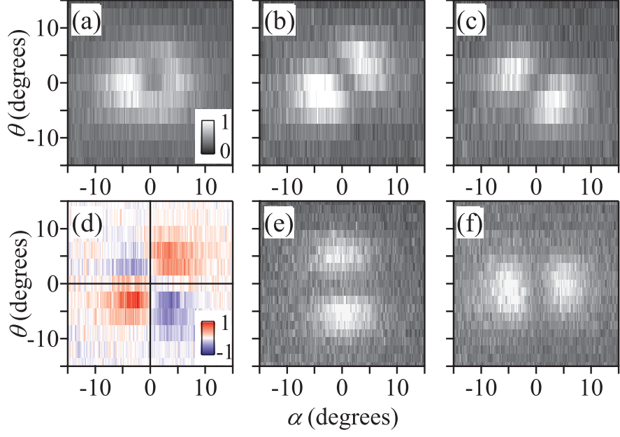
FIG. 4: (Color online) Spectral intensity distributions ( |E_B| \leq 5 meV) of SrTiO 3 :Nb recorded by various polarizations. (a) (I^+ + I^-)/2 . (b) I^+ . (c) I^- . (d) I^D showing sign change around \alpha = 0^\circ (vertical node) and \theta = 0^\circ (horizontal node). (e) I^s . (f) I^p .
