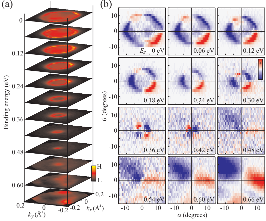
FIG. 5: (Color online) CDAD of Cu-doped \text{Bi}_2\text{Se}_3 . (a) Electronic structure recorded by ARPES on the (111) surface of \text{Cu}_x\text{Bi}_2\text{Se}_3 . Here, I^+ + I^- is converted into k -space map. The single crystal is grown from the melt. (b) I^D at various E_B 's. Also refer to a supplementary movie file.
