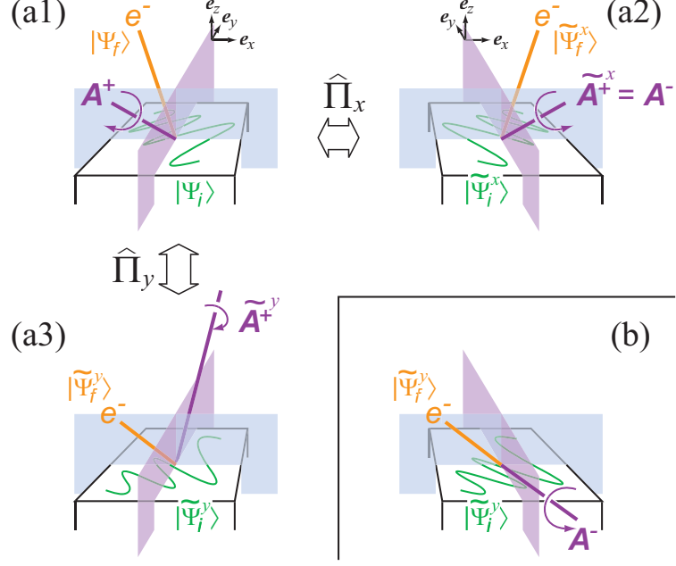
FIG. 2: (Color online) A bird's-eye view of photoemission. (a1) Photoemission by a right circularly polarized photon. (a2) and (a3) are mirror reflections of (a1) with respect to the x = 0 (incidence) plane and y = 0 plane, respectively. \hat{\Pi}_l ( l = x or y ) is the operator for the reflection with respect to the l = 0 plane, and we attach a tilde accompanied by l to the reflected states and the reflected vector potentials. (b) A configuration for achieving photoemission into |\tilde{\Psi}_i^y\rangle . Note the resemblance of (b) and (a3) up to the direction of the rotation of the vector potentials in the xy plane.
