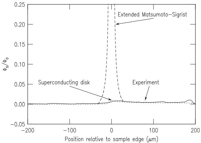
FIG. 5: Cross-section through the image of the ab face of \text{Sr}_2\text{CuO}_4 displayed in Figure 1 (solid line). The short-dashed line is the prediction for a superconducting disk in a uniform residual field of 3 nT. The long-dashed line (with a peak at \Phi_s/\Phi_0 = 1.1 ) is the prediction for a single domain p_x + ip_y superconductor of the extended-Matsumoto-Sigrist model as described in the text, assuming a square pickup loop 8\mu\text{m} on a side, at a height of 3\mu\text{m} above the sample. Here the superconductor is positioned to the left of 0\mu\text{m} , with epoxy to the right.
