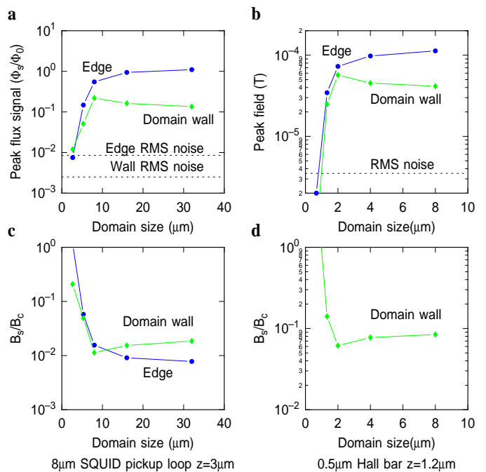
FIG. 8: a Plots of the predicted peak flux signals for an 8\ \mu\text{m} square SQUID pickup loop, 3\ \mu\text{m} above the sample surface, for a 64\ \mu\text{m} square p_x \pm ip_y superconductor with various domain sizes, using the predictions of Matsumoto and Sigrist 26 for the spontaneously generated edge and domain supercurrents. The dashed lines represent the estimated SQUID noise in the measurements within the sample (lower line) and at the sample edges (upper line). b Plots of the predicted peak fields for a square Hall bar 0.5\ \mu\text{m} on a side, 1.2\ \mu\text{m} above the sample surface, with the corresponding Hall bar noise floor. c Upper limits on the size of the scaling fields B_s , normalized by B_c = \Phi_0/2\sqrt{2}\pi\xi_0\lambda_L , as a function of domain size, given by our failure to observe spontaneously generated supercurrents at edges and domain walls in the SQUID measurements. In this figure the extended-Matsumoto-Sigrist predictions are represented by B_s/B_c=1 . d Upper limits on B_s/B_c as a function of domain size set by the Hall bar measurements.
