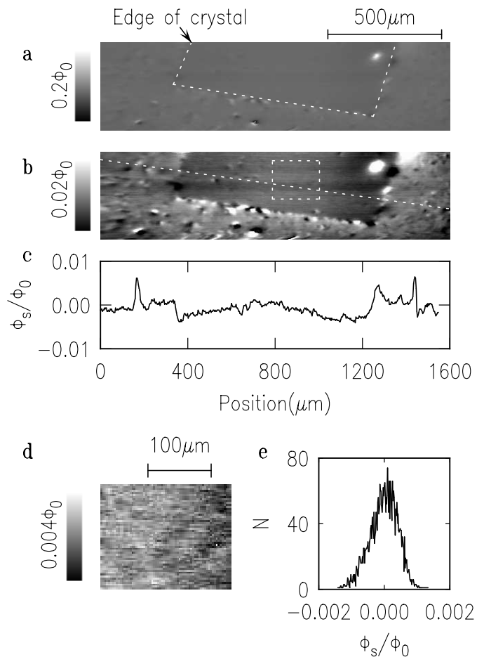
FIG. 1: SQUID microscope image of the ab face of a \text{Sr}_2\text{RuO}_4 single crystal, cooled in a field B_z < 10\ \text{nT} and imaged at T=0.27\text{K} with an 8\ \mu\text{m} square pickup loop. a Pseudocolor image with full-scale variation of 0.2\ \Phi_0 ( \Phi_0 = h/2e ) in magnetic flux through the SQUID pickup loop. The dashed line in a shows the outlines of the crystal. b Same image as a , but with the pseudocolor scale expanded to 0.02\ \Phi_0 . The dashed line in b shows the line traced by the cross-section in c . The dashed rectangle in b shows the area of the image expanded in d . e is a histogram of pixel values for the data displayed in d .
