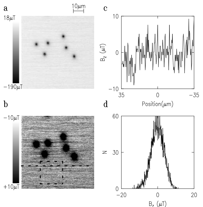
FIG. 4: a Scanning Hall bar image of ab face of \text{Sr}_2\text{RuO}_4 single crystal, cooled in \sim 2.5\ \mu\text{T} and imaged at a temperature below 100\text{mK} using a Hall bar with a sensor area 0.5\ \mu\text{m} on a side. In this image the mean of each scan line was subtracted from the raw data to remove slow drift in the sensor Hall voltage. b Same area as a but with an expanded pseudocolor scale. The dashed line in b shows the line traced by the data cross-section in c . The dashed square in b shows the area for which a histogram of pixel inductance values are displayed in d .
