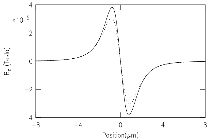
FIG. 9: Comparison of the predicted magnetic field sensed by a 0.5 \mu\text{m} square Hall bar, 1.2\mu\text{m} above a single domain in a p_x \pm ip_y superconductor, using the spontaneous domain currents predicted by Matsumoto and Sigrist, 26 with (dashed line) and without (solid line) surface screening effects as described in the text. The solid line corresponds to the extended-Matsumoto-Sigrist model.
