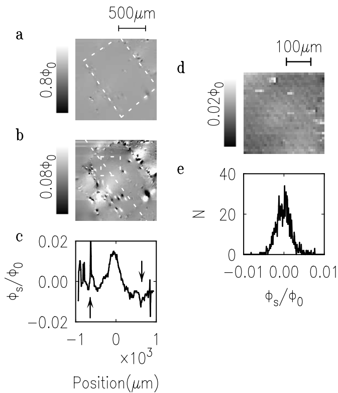
FIG. 3: SQUID microscope image of the ac face of a \text{Sr}_2\text{RuO}_4 single crystal cooled in nominally zero field and imaged at T=0.27\text{K} with an 8\ \mu\text{m} square pickup loop. a Pseudocolor image \Delta\Phi_s = 0.8\Phi_0 . The dashed line in a shows the positions of the outer edges of the crystal. b Same image as a , but with \Delta\Phi_s = 0.08\Phi_0 . A few interlayer vortices with both positive and negative signs are visible near the lower-left edge of the crystal. The dashed line in b is along the a -axis and shows the data traced by the cross-section in c . The arrows in c indicate the edges of the crystal. The dashed square in b shows the area of the image expanded in d . The diagonal stripes visible in d are due to 60 Hz noise. e is a histogram of pixel values for the data displayed in d .
