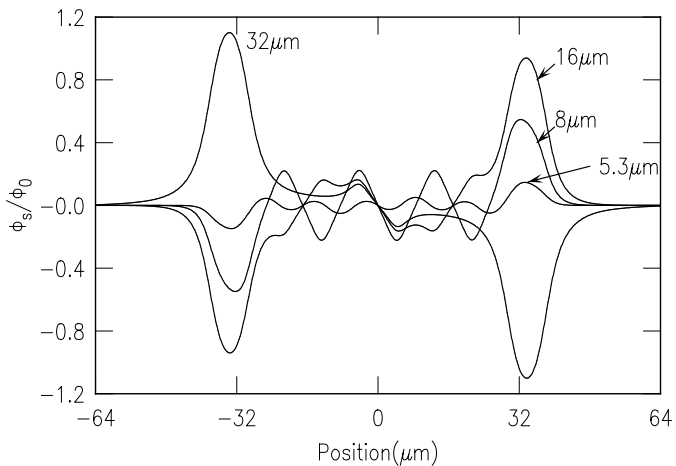
FIG. 7: Cross-sections through the modeling images of Fig. 6 for various domain sizes.
