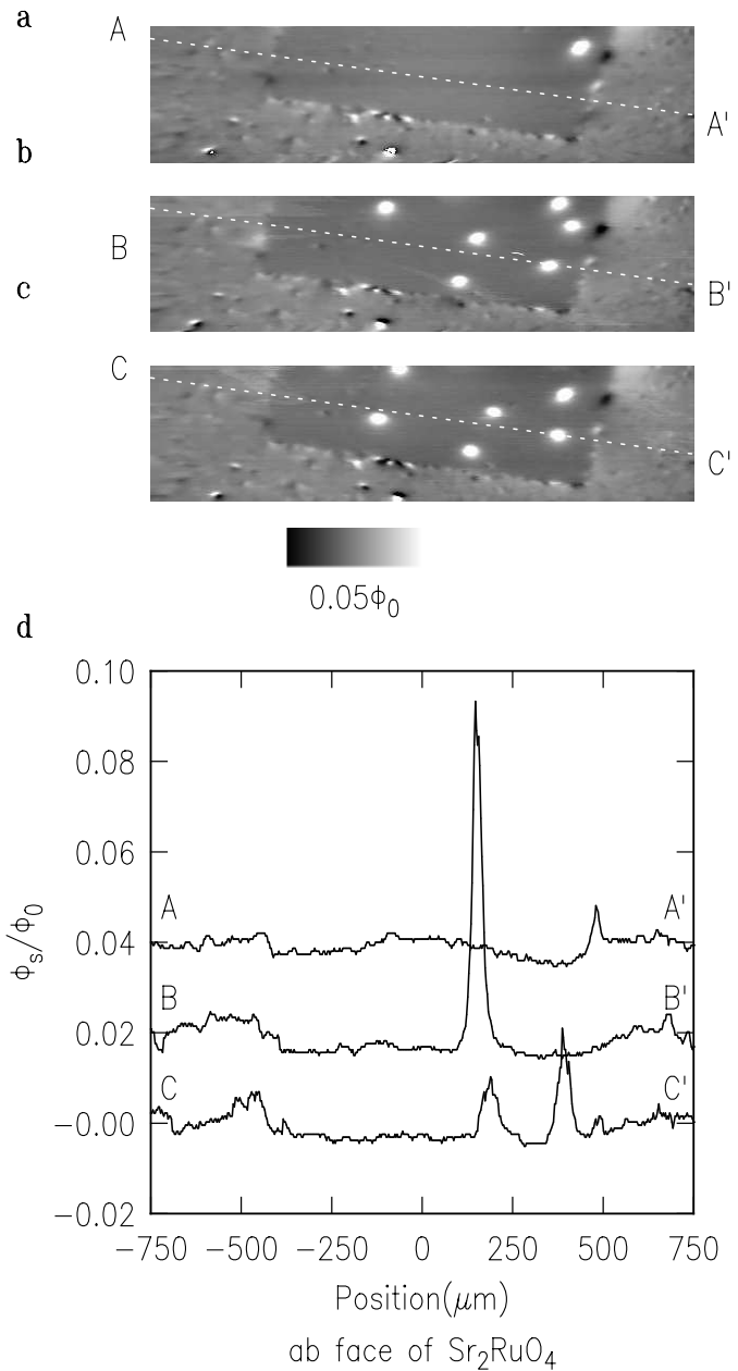
FIG. 2: Comparison of SQUID microscope images of an ab face of a \text{Sr}_2\text{RuO}_4 crystal after three different cooldowns in slightly different magnetic fields.
