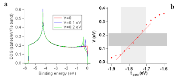
Fig. 25 : (a) Density of states in the TB model for indicated values of V ( t_{\text{para}}=-1.8\text{eV} and t_{\text{perp}}=0.35\text{eV} ). (b) Values of V stabilizing the CDW distortion as a function of t_{\text{para}} , assuming an elastic energy E=0.87*V^2 . Shaded area are ranges sampled by \text{RTe}_3 compounds.
