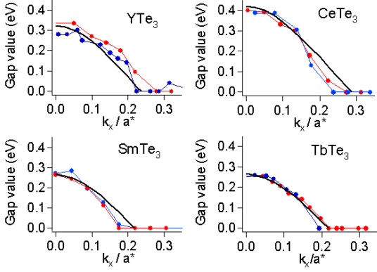
Fig. 13 : k -dependence of the gap along the Fermi Surface for the square part of FS (red points) and outer part (blue points). k_x is used as implicit parameter for the position on FS. The black line describes the decrease of the gap expected because of the imperfect nesting away from k_x=0 (see part III.D).
