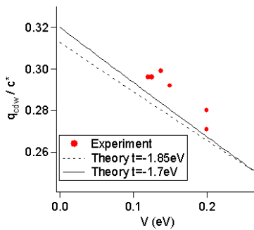
Fig. 20 : Red points : experimental values of q_{\text{cdw}} measured by x-ray (ref 17 and 16 for \text{CeTe}_3 ), as a function of V = \Delta/2 ( \Delta is taken from Fig. 14). Black lines : Theoretical variation for q_{\text{cdw}} as a function of V (see text), for t_{\text{para}} = -1.7\text{eV} and t_{\text{para}} = -1.85\text{eV} .
