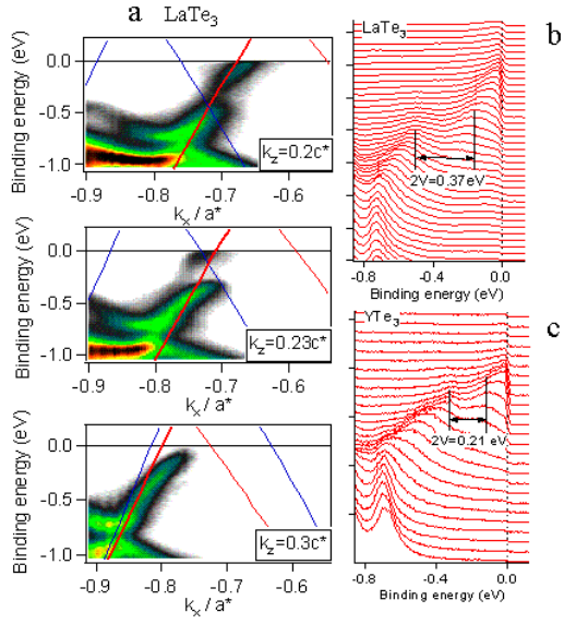
Fig. 18: (a) Dispersion along the outer FS in LaTe 3 for three k_z values ( h\nu=35 eV). The TB p_x band is shown as thick red line and CDW shadow bands as thin lines. (b) Detail of the dispersion in LaTe 3 at k_z=0.2c^* . (c) Equivalent situation for YTe 3 at k_z=0.32c^* (Fig. 10b).
