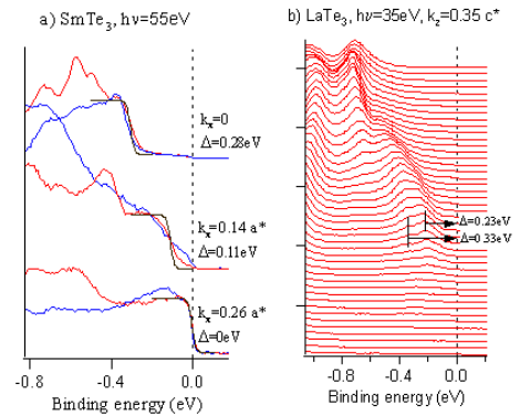
Fig. 21 : (a) Leading edge spectra in \text{SmTe}_3 at different k_x values and h\nu = 55\text{eV} on square part (red) and outer part (blue). The black line is a fitted Fermi step. (b) EDC spectra on the outer part in \text{LaTe}_3 at 35\text{eV} and k_z = 0.35c^* .
