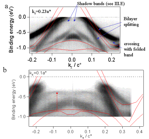
Fig. 9 : Near E_f band structure in the square. (a) Measured in \text{CeTe}_3 with photon energy of 55\text{eV} at k_x=0.23a^* and (b) in \text{TbTe}_3 with 35\text{eV} and k_x=0.1a^* . Red lines are calculated dispersions.
