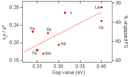
Fig. 22 : k_x^0 value at which the gap on FS becomes zero as a function of the maximum gap value. Samples are the same than in Fig. 14. Straight line is the position of k_x^0 calculated as a function of the gap value in the TB model. Right axis indicates the corresponding fraction of the FS contour that remains metallic.
