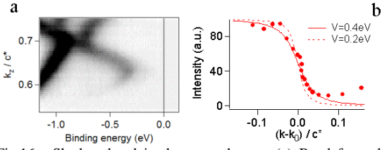
Fig.16 : Shadow band in the gapped state. (a) Band from the outer FS, measured along k_z at k_x=0.1a^* in CeTe_3 . (b) Red points : intensity of this band as a function of k (zero is the position of the crossing). It is extracted by a fit of the EDC spectra with a gaussian and a parabolic background. Theoretical variation for this weight is also shown for V=0.4eV (as solid line) and V=0.2eV (as dotted line).
