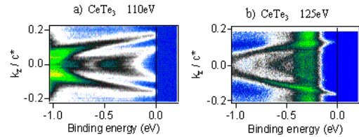
Fig. 7 : Comparison of the electronic structure, measured at T=20 K and k_x=0.6a^* , in \text{CeTe}_3 at a photon energy of (a) 110 eV and (b) 125 eV, i.e. respectively off and on the Ce 4d-4f resonance. The two parabolas come from the main and folded outer Te bands (see Fig. 8), the line at -0.28 eV in (b) is attributed to the spin-orbit satellite of the Ce resonance.
