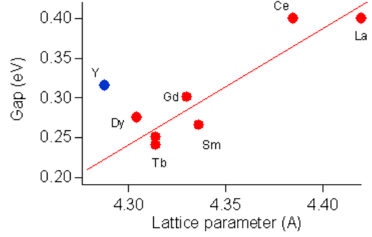
Fig. 14 : Maximum gap value for different rare-earths and \text{YTe}_3 (blue point), plotted as a function of the lattice parameter c . The straight line is a guide for the eyes.
