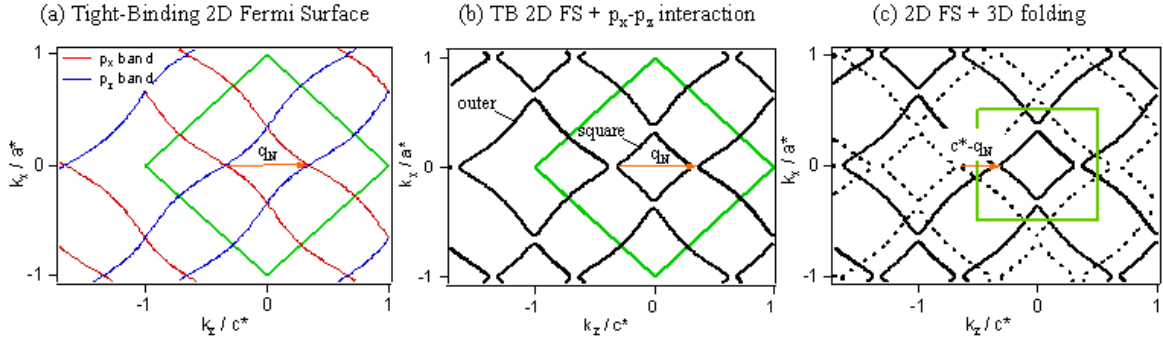
Fig. 4 : (a) Tight Binding FS for ( t_{\text{para}}=-1.7\text{eV} , t_{\text{perp}}=-0.35\text{eV} ) and ( t_{\text{para}}=-1.85\text{eV} , t_{\text{perp}}=-0.35\text{eV} ). The two contours overlap almost perfectly (see text). The green square delimits the BZ corresponding to one Te plane. The orange arrow represents the best nesting wave vector q_N . (b) Same as (a) after interaction between p_x and p_z that separates the "square" part of FS from the "outer" part. (c) Same as (b) plus, as dotted lines, the FS contours folded with respect to the 3D BZ limits (green square). The orange arrow represents the equivalent nesting direction, but defined in the 3D BZ : ( c^*-q_N ).
