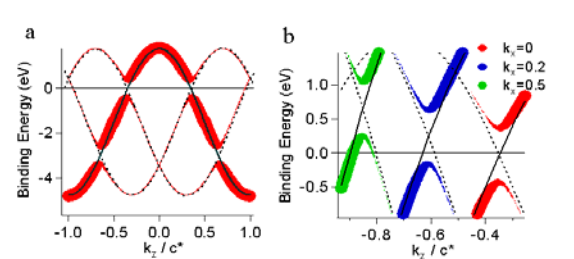
Fig. 15 : (a) Red points : sketch of the dispersion in the CDW state at k_x=0 , calculated for V=0.4\text{eV} and q_{\text{cdw}}=0.32c^* . The size of the points is proportional to the spectral weight |\psi|^2 (see text). The solid black line is the original dispersion from the TB model, dotted lines are translated by c^*\pm \mathbf{q}_{\text{cdw}} . (b) Zoom near the Fermi level for the same calculation and different k_x values.
