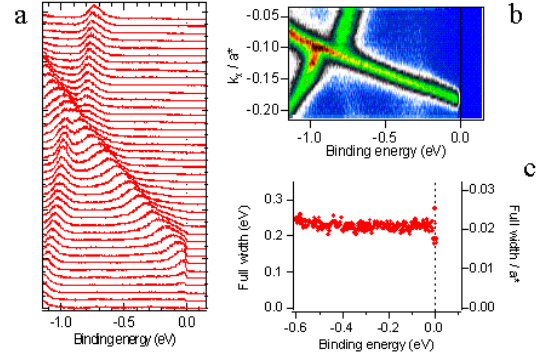
Fig. 12 : Lineshape analysis in \text{CeTe}_3 at 55eV and 20K for a cut of the outer FS at k_x=0.62c^* . (a) EDC stacks. (b) Image plot. (c) Full width at half maximum of MDC spectra (the value in energy is obtained by multiplying with the slope of dispersion).
