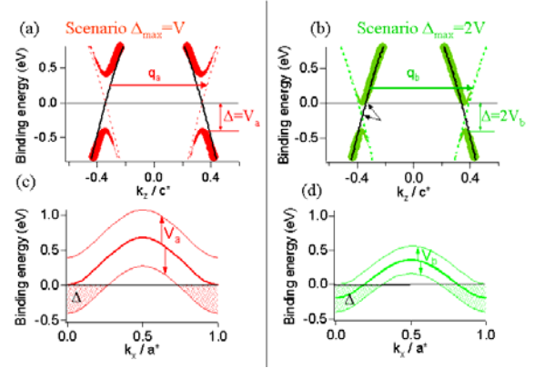
Fig. 19 : (a) and (b) : Black line is the TB band at k_x=0 , dotted lines are translated by \pm q , with q_a=0.68c^* and q_b=0.733c^* . V is chosen to get the same gap in the two cases : V_a=0.4 eV and V_b=0.2 eV. (c) and (d) : Thick line is the position of the crossing between the original and translated bands as a function of k_x , for the values of q and V corresponding to (a) and (b). Thin lines are translated by \pm V . Dotted areas represent the gapped regions.
