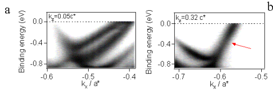
Fig. 10 : Near E_f band structure along the outer FS measured in YTe_3 in the 2 nd BZ (see Fig. 8) at 35eV, for (a) k_z=0.05c^* and (b) k_z=0.32c^* .
