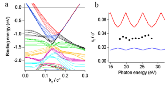
Fig. 11 : (a) Calculated band dispersion at k_x=0.3a^* , for different k_y values. (b) Black points : k_f position measured in CeTe_3 for the square as a function of photon energy. Solid lines : perpendicular dispersion expected theoretically on the square for the red and blue bands of panel (a).
