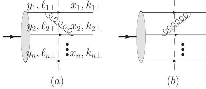
FIG. 1: Light-front time-order perturbation Feynman diagrams for the phase contribution from one-gluon exchange between two constituent quarks.
