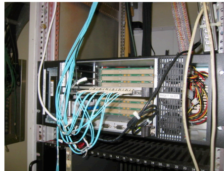
Fig. 8. The system is presently using the micro-PC to control the DAQ. Only two slots are occupied at present.
