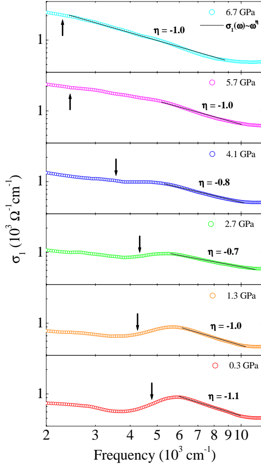
FIG. 3: (color online) Real part \sigma_1(\omega) of the complex optical conductivity of LaTe 2 at various pressures, plotted on a bi-logarithmic scale. The arrows indicate the position of \omega_{SP} (eq. (3)). The power-law behavior ( \sigma_1(\omega) \sim \omega^\eta ) is also displayed with the resulting exponent \eta .
