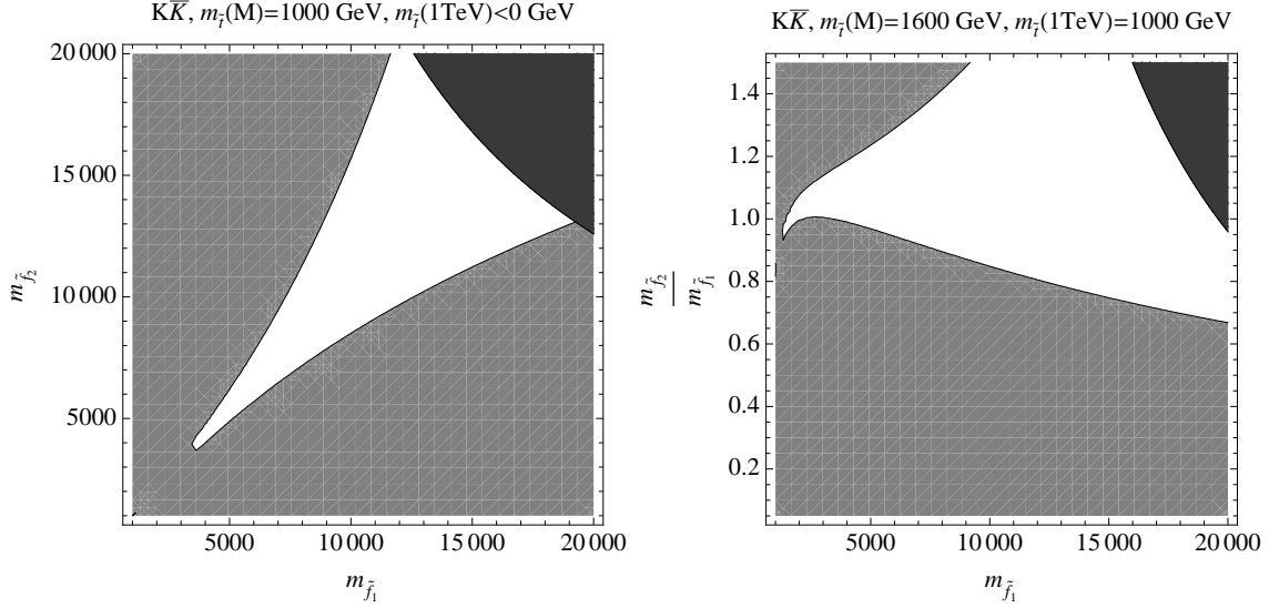
Figure 1: Constraints on first and second generation sfermion masses. Light gray region ruled out by K - \bar{K} -mixing. (a) Dark gray region ruled out by tachyonic stops at the weak scale ( m_{\tilde{t}}(1 \text{ TeV}) < 0 ). We assumed m_{\tilde{g}} = 500 \text{ GeV} , m_{\tilde{t}}(100 \text{ TeV}) = 1 \text{ TeV} . Note that the stop mass constraint disappears completely for the m_{\tilde{f}_1} and m_{\tilde{f}_2} mass range shown when m_{\tilde{t}}(100 \text{ TeV}) \gtrsim 1.6 \text{ TeV} . (b) Dark gray region ruled out by stops being too light at the weak scale to give a Higgs mass above LEP limits ( m_{\tilde{t}}(1 \text{ TeV}) \lesssim 1000 \text{ GeV} , assuming the trilinear coupling is negligible). We assumed m_{\tilde{g}} = 500 \text{ GeV} , m_{\tilde{t}}(100 \text{ TeV}) = 1.6 \text{ TeV} .
