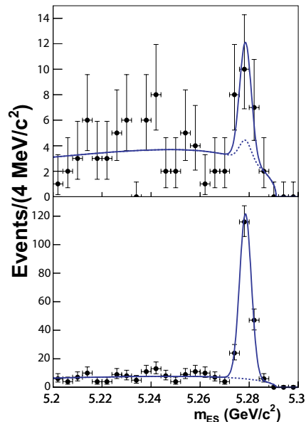
FIG. 4: Distributions of m_{ES} for the wrong-sign (top) and right-sign (bottom) decays. These decay categories are defined in the text. The dashed curve indicates the total background contribution. It also includes the right-sign peaking background estimated from a Monte Carlo study for the wrong-sign (top) decays. The curves result from a simultaneous fit to these distributions with identical PDFs for both samples.
