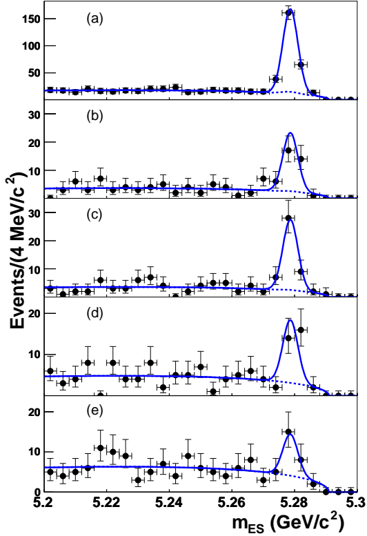
FIG. 2: Distributions of m_{ES} in the signal region for (a) the non- CP modes in B^\pm decays, (b) the CP+ modes in B^+ , and (c) B^- decays and (d) the CP- modes in B^+ and (e) B^- decays. The dashed curve indicates the total background contributions, which include the fake D backgrounds.
