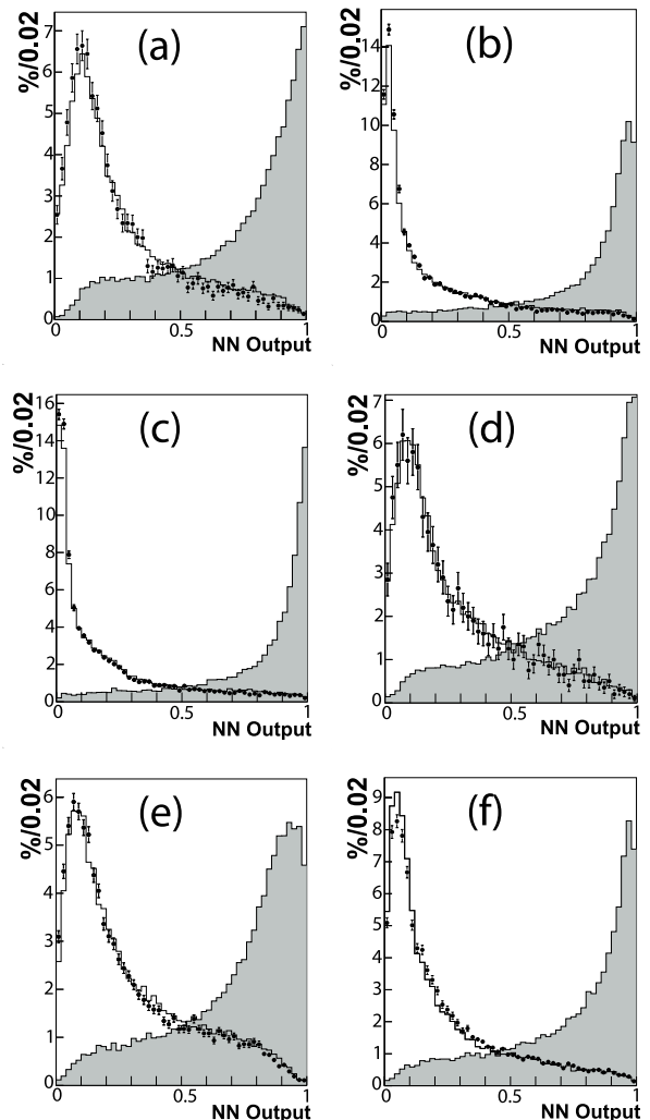
FIG. 1: Neural network (NN) outputs and results of the NN verifications of (a) K^+K^- , (b) \pi^+\pi^- , (c) K_s^0\pi^0 , (d) K_s^0\phi , (e) K_s^0\omega , and (f) K^-\pi^+ subsamples of the GLW analysis. The samples used to produce the output are shown as histograms. The signal (Monte Carlo simulation) is the shaded histogram peaking near 1; the continuum (Monte Carlo simulation) is the histogram peaking near 0. The off-peak data used to check the NN are overlaid as data points.
