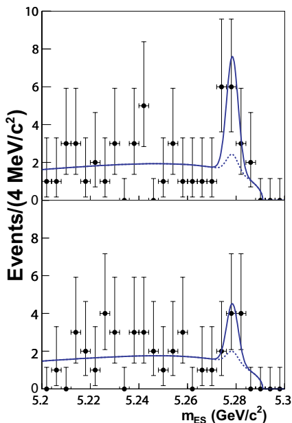
FIG. 5: The wrong-sign sample shown in the top plot of Fig. 4 split by charge. Upper plot shows the m_{ES} distribution of the B^+ \rightarrow [K^-\pi^+]_D K^{*+} decays while lower plot presents the same for the B^- \rightarrow [K^+\pi^-]_D K^{*-} decays. The dashed curve indicates the total background contribution which includes the right-sign peaking background.
