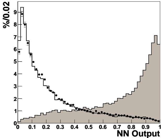
FIG. 3: Neural network (NN) output and result of the NN verification for the ADS analysis (see text). The samples used to produce the output are shown as histograms. The signal (Monte Carlo simulation) is the shaded histogram peaking near 1; the continuum (Monte Carlo simulation) is the histogram peaking near 0. The off-peak data used to check the NN are overlaid as data points.
