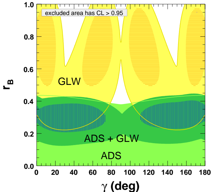
FIG. 6: 95% confidence level contours from a two dimensional scan of \gamma versus r_B from the B^- \rightarrow DK^{*-} GLW and ADS measurements. Also shown are the 68% confidence level regions (striped areas) for the GLW and the fit which uses both the GLW and ADS measurements. r_D and \delta_D are from Ref. [12].
