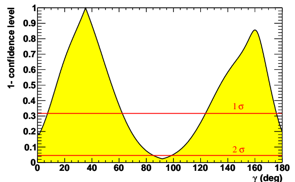
FIG. 8: Constraints on \gamma from a fit which uses both the B^- \rightarrow DK^{*-} GLW and ADS measurements as well as r_D and \delta_D from [12]. The horizontal lines show the exclusion limits at the 1 and 2 standard deviation levels.
