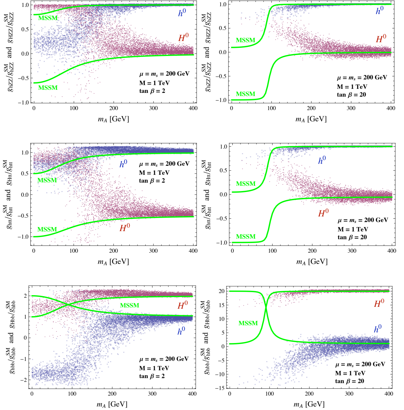
Figure 6: Tree-level couplings of the CP-even Higgs states (normalized to the SM ones) to gauge bosons (upper plots), to top pairs (middle plots) and to bottom pairs (lower plots), as a function of m_A , for \tan\beta = 2 (left panels) and \tan\beta = 20 (right panels). The blue crosses correspond to the couplings of h , and the red dots to those of H . The solid green lines correspond to the tree-level MSSM result. The region of parameter space in the scan is described in the main text.
