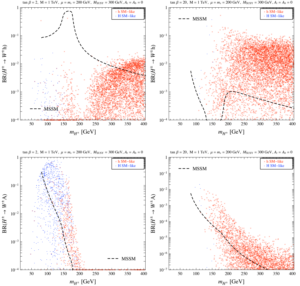
Figure 11: Branching fractions for H^\pm \rightarrow W^{\pm(*)}h (upper panels) and H^\pm \rightarrow W^{\pm(*)}A (lower panels), for \tan \beta = 2 (left panels) and \tan \beta = 20 (right panels). The dashed line corresponds to the MSSM result. SUSY and QCD radiative corrections are included. We indicate by red crosses those points where h is SM-like ( |g_{hZZ}| > |g_{HZZ}| ) and by blue dots those points where H is SM-like ( |g_{HZZ}| > |g_{hZZ}| ).
