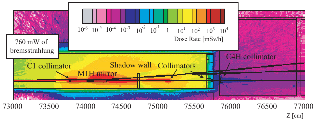
Figure 2: Two dimensional view of the rate inside the FEE and first experimental hutch due to the use of a beam finder wire for the maximum allowed nominal beam power.
