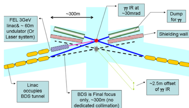
Figure 1: Conceptual configuration of Beam Delivery System, tunnels and location of FEL for the first 180GeV CM \gamma\gamma stage of a staged linear collider [7].
