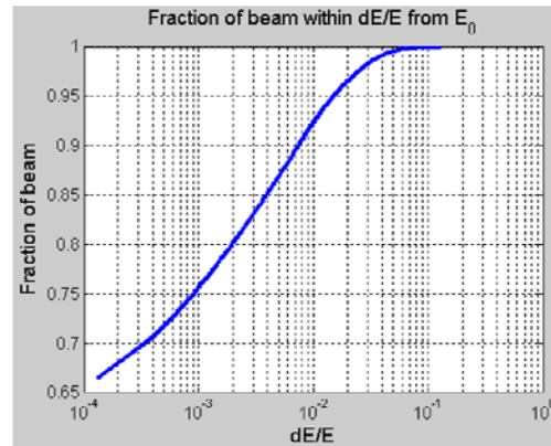
Figure 5: Cumulative distribution of disrupted beam for an academic exercise energy recycle parameter set.
