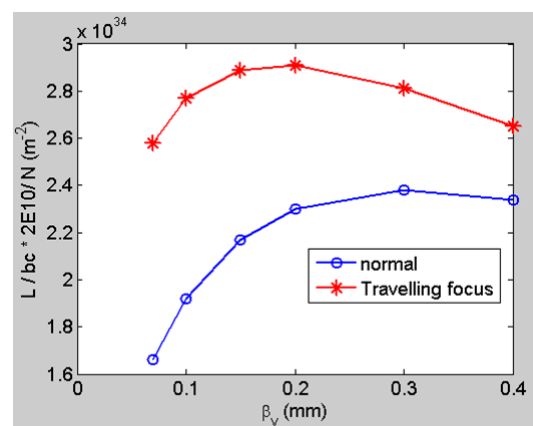
Figure 1: Hour-glass and travelling focus.
