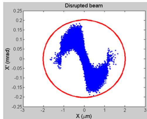
Figure 6: X-X' for disrupted beam of E-recycle set. The red circle corresponds to 200mm*mrad emittance.
