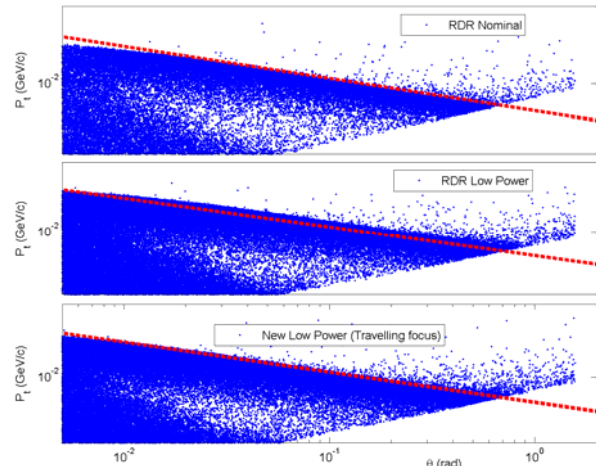
Figure 4: Distribution of e+e- pairs.
