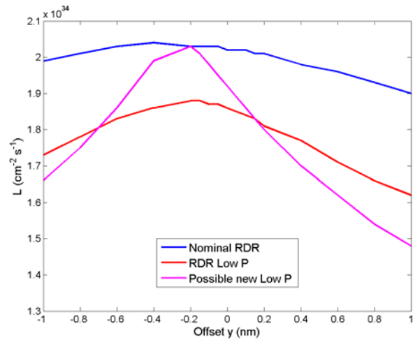
Figure 3: Luminosity versus beam offsets.
