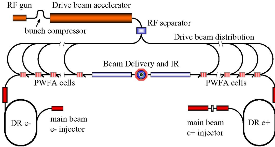
Figure 1: Concept for a multi-stage PWFA-based Linear Collider.
