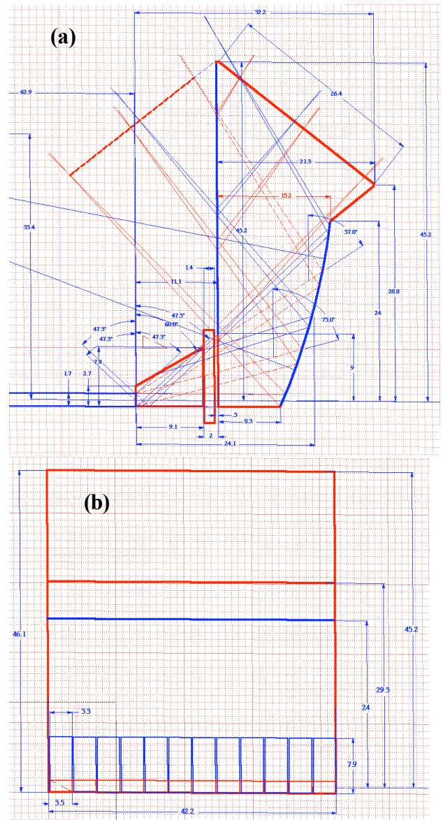
Fig. 2. (a) A side view of the FDIRC focusing block with a cylindrical and flat mirrors, and focal plane. The cylindrical mirror radius is 90 cm, with a center at (z_{center} = 62.9 \text{ cm}, y_{center} = 35.4 \text{ cm}) . (b) A front view of the of the FDIRC focusing block and 12 wedges and bars. This design corresponds to a file: FDIRC_SOB_design_3a.vc6.
