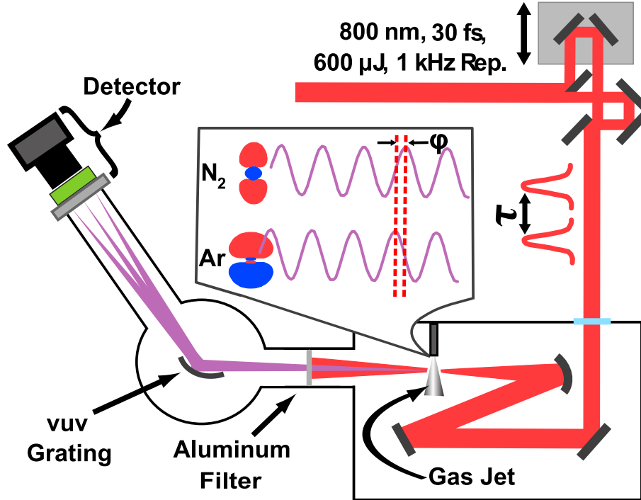
FIG. 1: (Color online) High Harmonic Generation setup. The laser beam is split into time delayed pump-and probe pulses in a pulse front beam splitter. The two beams are recombined on a molecular jet from a supersonic expansion in vacuum. One pulse aligns the sample, and the other one creates high harmonics on the aligned sample. The high harmonics are dispersed in a vuv spectrometer and detected on an MCP-phosphor screen assembly.
