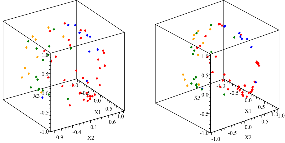
Figure 5: The left hand picture is the raw data from the Affymetrix Chip plotted for principal components 2,3,4. Clearly, without the coloring it would be hard to identify clusters. The right hand picture is the same data after DQC evolution using \sigma = 0.2 and a mass m = 0.01 . The different classes are shown as blue, red, green and orange.
