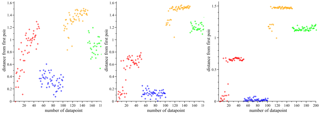
Figure 3: A plot of Euclidean distance of each point i from the first data point. Again, the left hand plot shows the distances for the initial distribution of points. The middle plot shows the same distances after quantum evolution. The right-hand plot shows results after another iteration of DQC. The numbering of the data-points is ordered according to the expert classification of these points into four classes containing 50 instances each.
