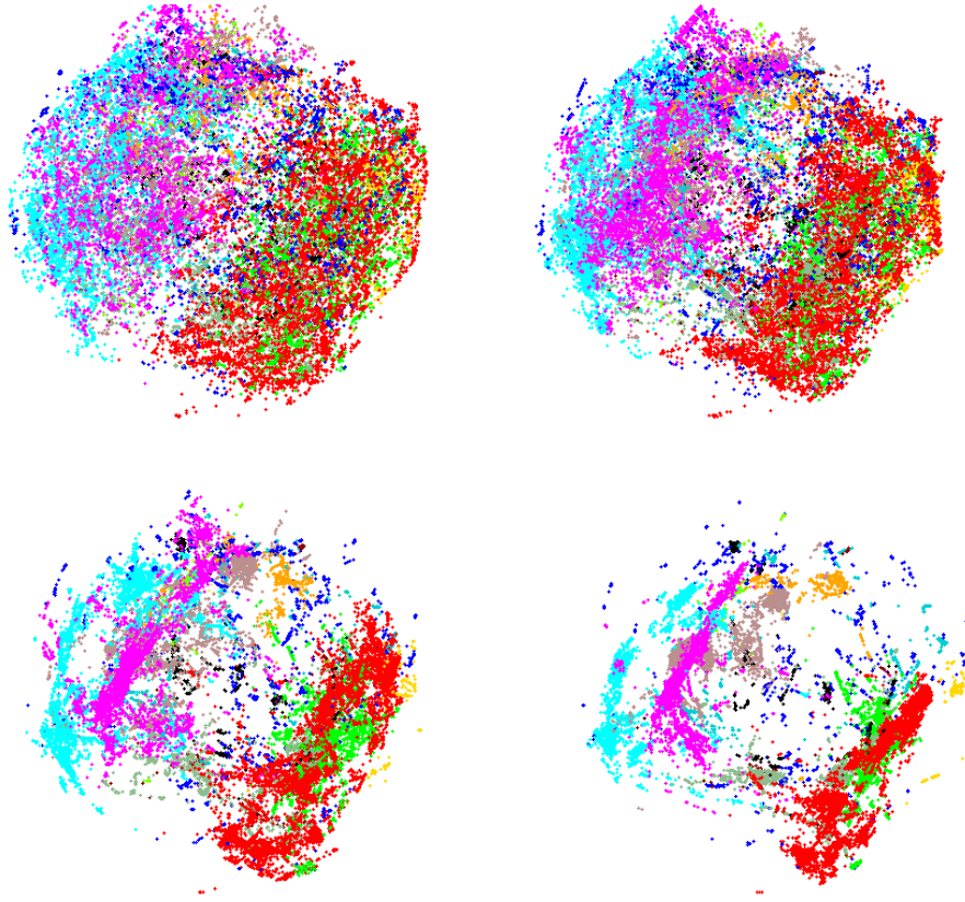
Figure 4: A plot of the first three principal components for a large data-set, comprising 35,213 points in 20 dimensions, before and after DQC evolution. The potential was determined from the full data-set and evolved using a sub-set of 1200 points, whose Gaussians serve as an essentially linearly set of independent states. Three stages of DQC development are shown. The coloring was decided upon by selecting the most obvious clusters from the evolved data and assigning colors to them. The dark blue points correspond to points that we did not bother to assign to clusters. The purpose of coloring is to be able to look at the points in the original data, discern those that belong to common structures, and follow their dynamic distances under DQC evolution.
