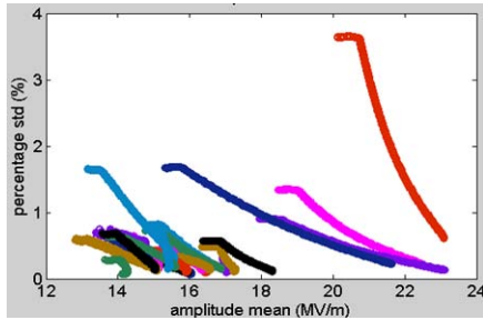
Figure 5: PSD of all cavity probe signals at each sample point during the flattop period as a function of gradient.
