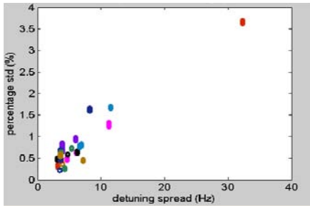
Figure 6: Correlation between cavity probe PSD and detuning ASD at the end of the flattop.
