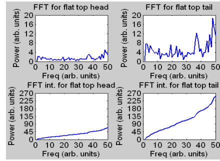
Figure 7: FFT and integrated FFT of for ACC6-CAV1.
