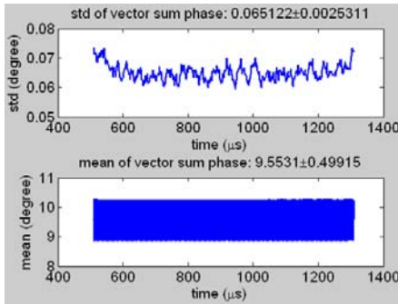
Figure 2: ASD and mean VS phase for the flattop.
