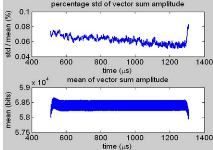
Figure 1: PSD and mean VS amplitude for the flattop.
