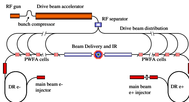
Fig. 1: Concept for a multi-stage PWFA Linear Collider.
