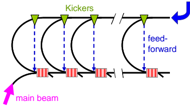
Fig. 3: Drive beam distribution system and PWFA cells.
