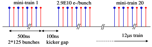
Fig. 4: Drive beam train configuration.
