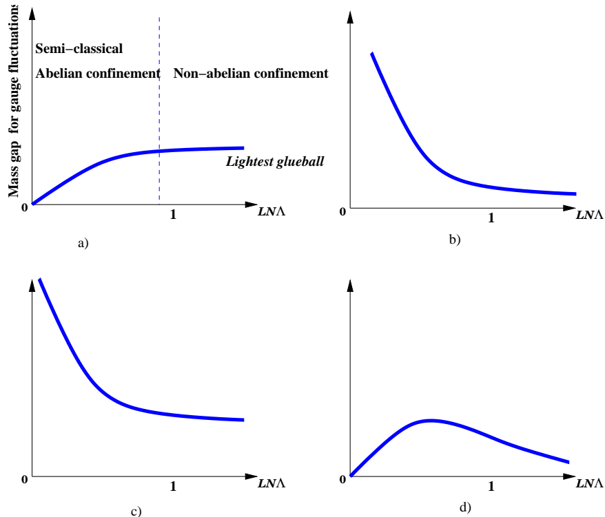
Figure 1: Possible behavior of the mass gap for gauge fluctuations in asymptotically free, center-symmetric theories as a function of the radius of \mathbf{S}^1 : a.) N_f small: mass gap increases in the semiclassical domain of abelian confinement and saturates to its \mathbf{R}^4 value in the non-abelian confinement domain. b.) N_f sufficiently large, perhaps just below N_f^{AF} : mass gap is a decreasing function of radius. There are theories in this class for which semiclassical analysis applies at any size \mathbf{S}^1 . c.) Mass gap may start decreasing in the semiclassical domain, but may possibly saturate to a finite value on \mathbf{R}^4 . This may happen, for example, if \chi SB takes place on the way. d.) Mass gap starts to increase in the semiclassical domain, but before reaching \Lambda L \sim 1 , the coupling reaches a fixed point value without triggering \chi SB and the mass gap decreases to zero at larger scales. We will argue that a.) and b.) occur at small and large N_f , respectively, in all classes of theories we consider. We do not know whether c.) and d.) occur in any of the theories we consider and our semiclassical methods are of no help in this regard. We note, however, that c.) and d.) are mutually exclusive—if either kind of behavior exists in a given class of theories for some N_f , the other kind is not expected to occur, see the text.
