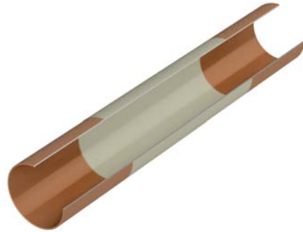
Figure 5: Cylindrical insert of higher resistivity in a round pipe.
