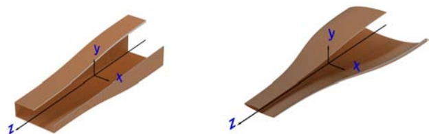
Figure 1: Smooth tapers with rectangular (a) and elliptic (b) cross sections.
