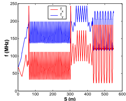
Fig. 2: The CO^+ frequency along quarter of the ring, 5% coupling
