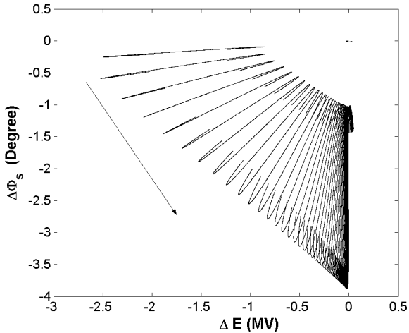
Figure 6: Example of development of phase space of different bunches. Each bunch is presented by one dot. The line-like shape gives the phase-space of all bunches at different time.
