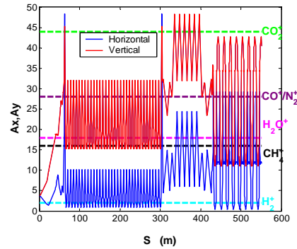
Fig. 1: Critical mass number for 5% coupling. The mass number of H_2 , CH_4 , H_2O , CO and CO_2 is marked in the plot.
