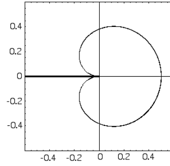
Figure 2: Stability diagram for the galaxy distribution.
