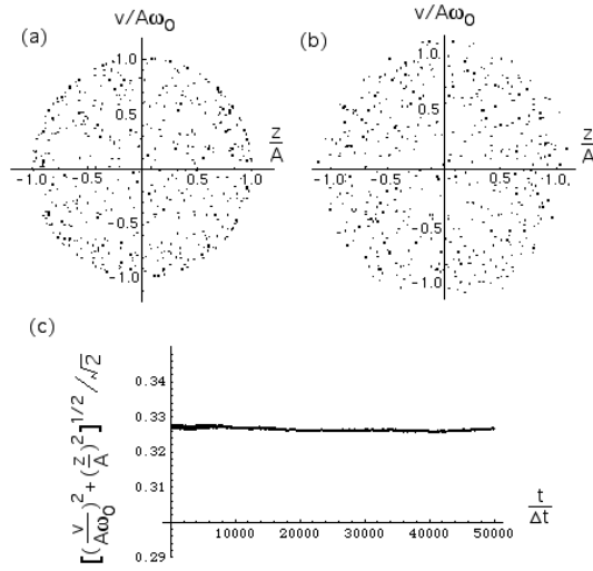
Figure 6: Simulation result of a 1-D nonrotating galaxy model. (a) Initial phase space distribution of 500 stars, (b) Final distribution after 2000/2\pi periods, (c) Plot of galaxy emittance \sqrt{[(v/\omega_0 A)^2 + (z/A)^2]}/\sqrt{2} as a function of the step number t/\Delta t , showing no sign of instability.
