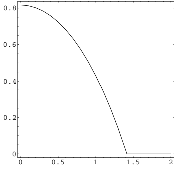
Figure 3: v vs u according to Eq.(18).
