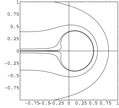
Figure 4: Contours of constant growth rates.
