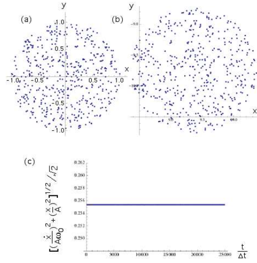
Figure 7: Simulation result of the 2-D rotating galaxy. (a) Initial distribution of 500 stars in the x - y space, (b) Final distribution after 1000/2\pi periods, (c) Plot of galaxy emittance \sqrt{[(x/A)^2 + (\dot{x}/\omega_0 A)^2]}/\sqrt{2} as a function of the step number t/\Delta t , showing no sign of instability.
