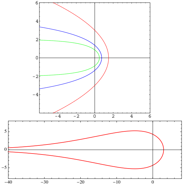
Figure 5: Upper: Stability diagrams for galaxy distributions are plotted in red, blue, green for Cases 1, 2, 3, respectively. Lower: Case 4.
