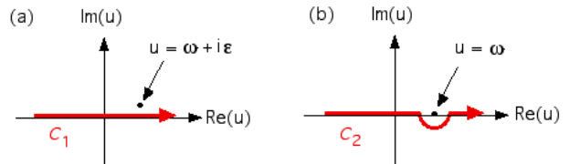
Figure 1: Integration contour dictated by Landau damping analysis.
