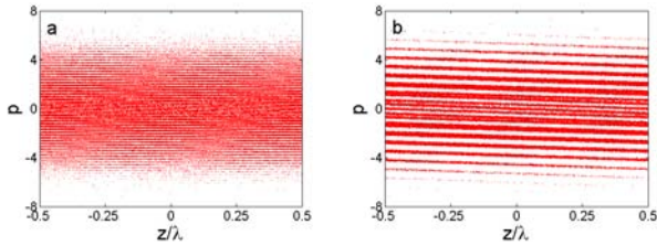
Figure 1: Longitudinal phase space at the exit from the first dispersion section for the case A_2 = 1 (a) and A_2 = 3 (b).
