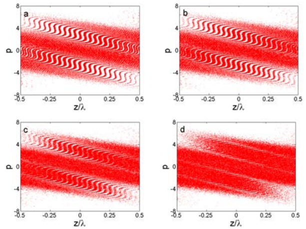
Figure 2: Longitudinal phase space at the exit of the second dispersion section for various R_{51} : (a) R_{51}\sigma_x = 0.05\lambda_r ; (b) R_{51}\sigma_x = 0.1\lambda_r ; (c) R_{51}\sigma_x = 0.2\lambda_r ; (d) R_{51}\sigma_x = 0.5\lambda_r .
