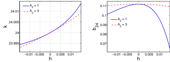
Figure 4: (a) Harmonic number at various energy chirp; (b) Bunching factor at various energy chirp.
