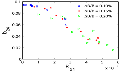
Figure 3: Bunching factor vs R_{51} for various field errors. The standard deviation of \Delta B/B indicated in the plot.
