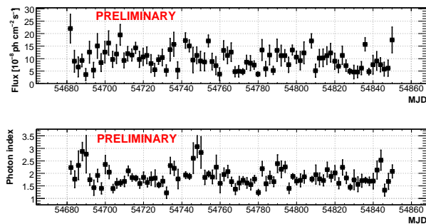
Fig. 2: \gamma -ray flux at E > 0.2 GeV (top) and spectral photon index from a Power Law fit (bottom) from Mrk421 for 2-day time bins from 4 August 2008 to 20 January 2009. Vertical bars denote 1 \sigma uncertainties.
