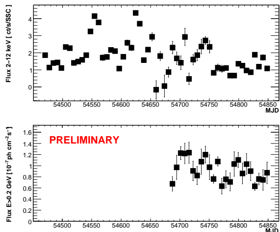
Fig. 1: Light curves from Mrk421 with weekly time bins since 1 January 2008 obtained with two all-sky-monitoring instruments: RXTE/ASM (2-12 keV, top figure), and Fermi-LAT (at E > 0.2 GeV, bottom). Vertical bars denote 1 \sigma uncertainties.
