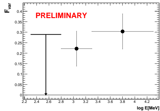
Fig. 3: Fractional variability parameter as derived for 3 energy bins according to [10]. The variability was computed using the fluxes on week time scales. Vertical bars denote 1\sigma uncertainties, horizontal bars indicate the width of each energy bin. The arrow indicates 95% confidence level upper limits on the fractional variability.
