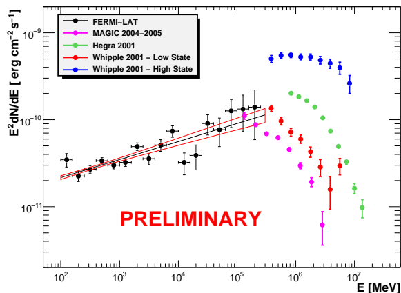
Fig. 4: Spectral energy distribution of the MRK421. Black line is the likelihood PL fit; red contour is 68% uncertainty of the fit; data points: (black) Fermi-LAT data; TeV observations: Whipple in a high state (blue) and low state (red) of the source during 2001, Hegera in 2001 (green) and MAGIC in 2004-2005 (pink).
