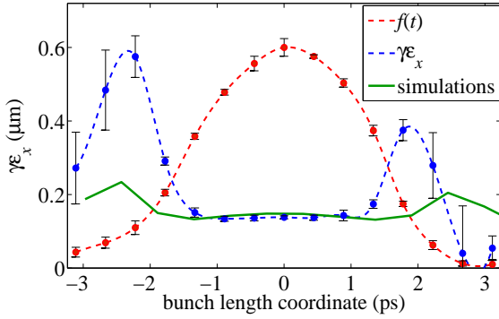
Figure 2: Measured (blue dots) and simulated (green curve) time-sliced horizontal emittance along the length of the bunch at a charge of 20 pC. Smooth curves on the measured data aid the eye and f(t) is the measured bunch temporal distribution on an arbitrary scale.
