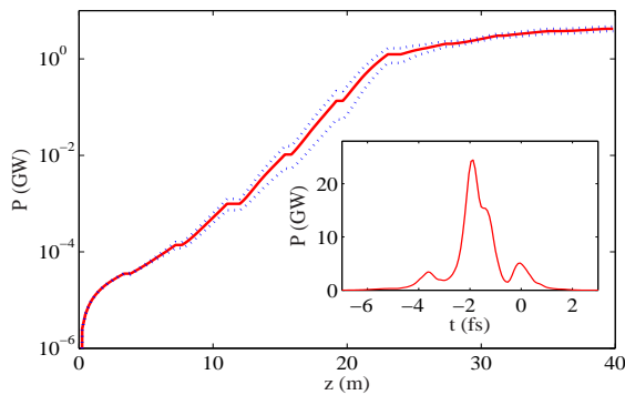
Figure 5: Genesis simulation at 15 Å. The average FEL power (solid line) and the rms fluctuation (dashed lines) along the undulator. The inset plot shows a snapshot of a typical 2-fs FEL pulse at 25 m (inset). The RF phase of L2-linac is -35.5^\circ and L3-linac is switched off in simulations.
