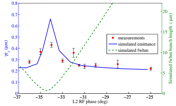
Figure 3: Measured (red circles) and simulated (blue curve) projected emittance at 10 GeV versus L2-linac RF phase with a bunch charge of 20 pC. Simulated bunch length (green dashed curve) also shown at the right axis.
