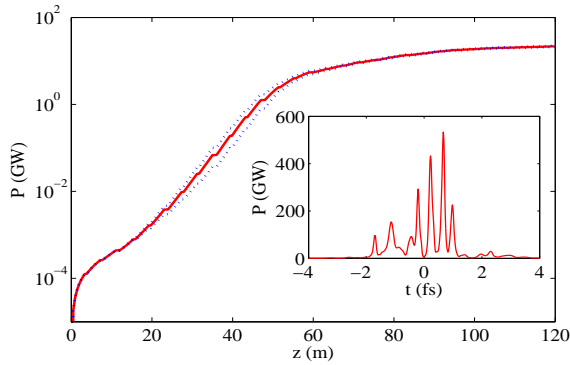
Figure 4: Genesis simulation at 1.5 Å. The average FEL power (solid line) and the rms fluctuation (dashed lines) along the undulator. The inset plot shows a snapshot of a typical 2-fs FEL pulse at 100 m. The RF phase of L2-linac is -35^\circ in simulations.
