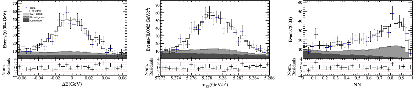
FIG. 3: Distributions of \Delta E (left), m_{ES} (center), and NN output (right) for a sample enhanced in B^0 \rightarrow K_S^0 \pi^+ \pi^- signal with a requirement on the likelihood ratio R computed without the variable being plotted. In each case the applied cut rejects 99% of continuum background, while retaining 28% of signal for \Delta E and m_{ES} , and 16% for NN . A veto in the D^- \pi^+ and J/\psi K_S^0 bands has been applied.
