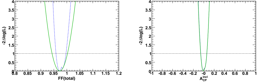
FIG. 14: Statistical (dashed line) and total (solid line) scans of -2\Delta \log \mathcal{L} as a function of the total fit fraction (left) and the inclusive direct CP -asymmetry A_{CP}^{incl} (right). A horizontal dotted line marks the one standard deviation level.
