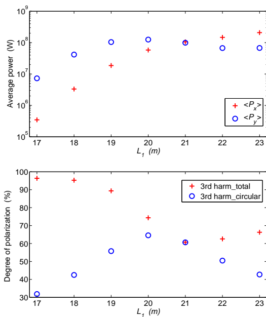
Figure 2: Power and degree of polarization of the third harmonic radiation using Method I.
