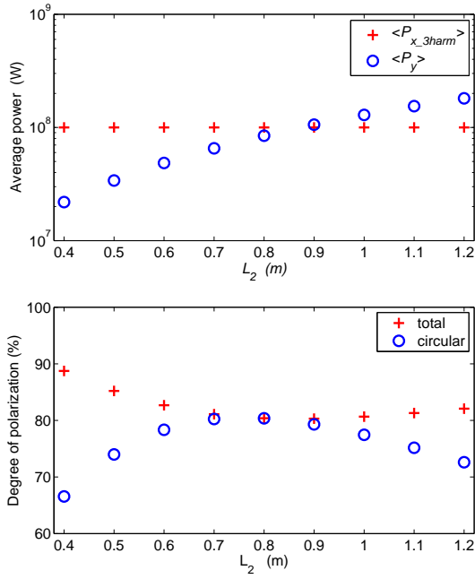
Figure 3: Power and degree of polarization of the third harmonic using Method II.
