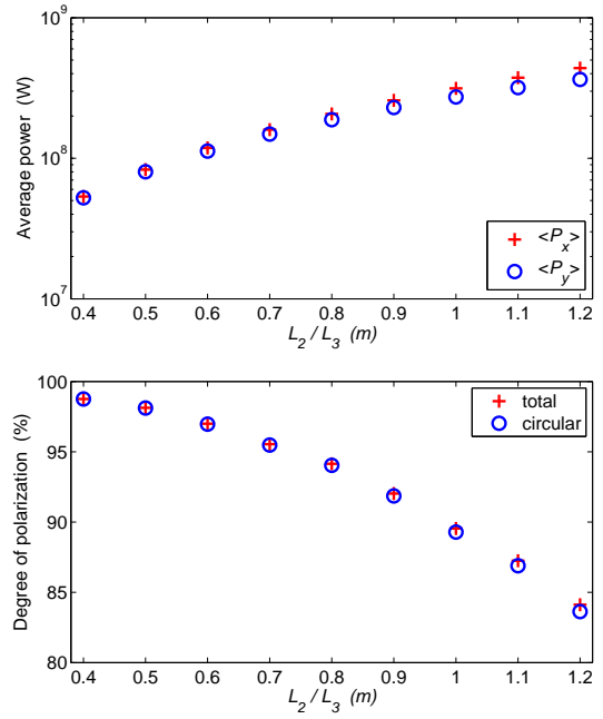
Figure 4: Power and degree of polarization at the second harmonic using our modified crossed undulator scheme.
