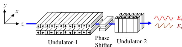
Figure 1: A sketch of crossed undulators for polarization control.
