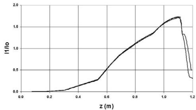
Figure 6: Fundamental bunching I_1/I_0 for 1D, 2D and 3D codes are virtually identical
