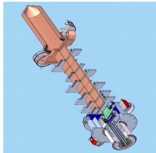
Figure 1: SBK Design.
