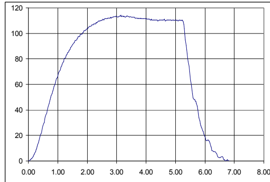
Figure 13: kV vs. microseconds for the modulator pulse into an 850 \Omega load
