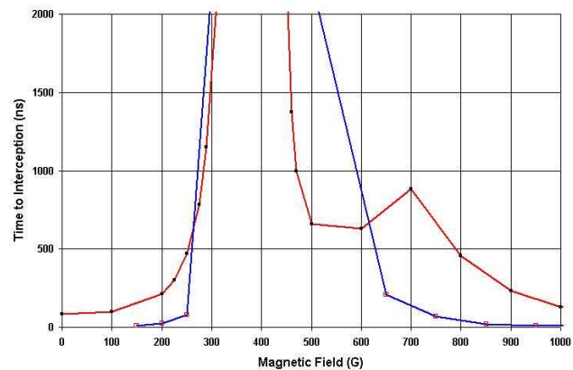
Figure 11: Stability curve of a 2-cavity PCM system (2D-red curve, 3D-blue curve)
