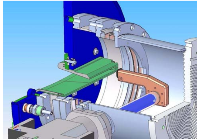
Figure3: BSD Cutaway.
