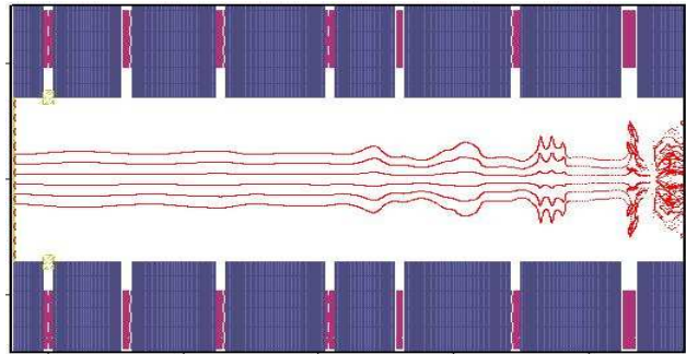
Figure 10: 10 MW 390 G-780 G solenoid design
