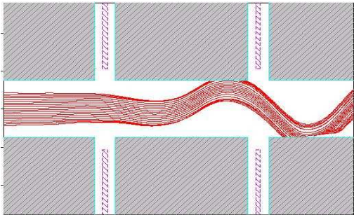
Figure 8: Side view of the 2-Cavity oscillation disrupting beam transport, PCM Brillouin.
