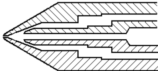
Figure 4: BSD tip. cross section
