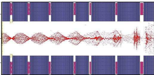
Figure 9: 10 MW 390 G RMS PCM design
