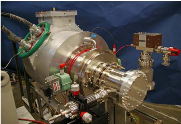
Figure 12: BSD mounted to small oil tank and connected to modulator
