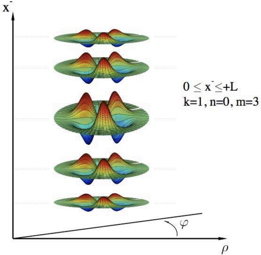
FIG. 5: (color online) Transverse sections of a 3-D basis function involving a 2-D harmonic oscillator and a longitudinal mode of Eq. 5 with box boundary conditions (wavefunction vanishes at \pm L ). The quantum numbers for this basis function are given in the caption. The basis function is shown for positive values of x^- and is antisymmetric with respect to x^- = 0
