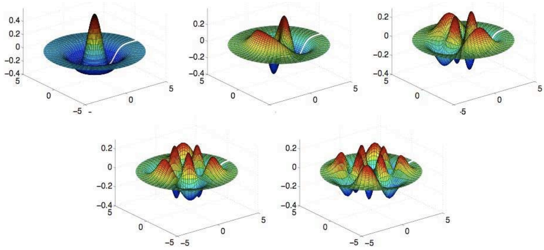
FIG. 3: (color online) Modes for n = 1 of the 2-D harmonic oscillator selected for the transverse basis functions. The orbital quantum number m progresses across the rows by integer steps from 0 in the upper left to 4 in the lower right and counts the pairs of angular lobes.
