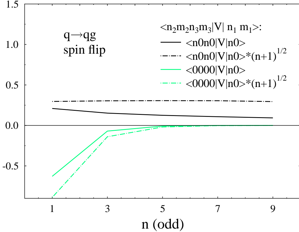
FIG. 14: (color online) Behavior of representative fermion to fermion-boson matrix elements in BLFQ. The quantum numbers specifying the parton transverse modes (n_i, m_i) in the matrix elements are given in the legend. Only the transverse mode contributions to the matrix elements are shown. Results are also shown with a multiplicative factor of \sqrt{n+1} applied to identify logarithmic divergence by a resulting flat behavior, when it occurs. Note that for one of the cases shown, the resulting matrix elements vanish with increasing n while the other case shows a constant trend but does not enter a second-order perturbative analysis. Overall matrix element normalization depends on the specific values of light-front momentum fractions carried by the interacting partons.
