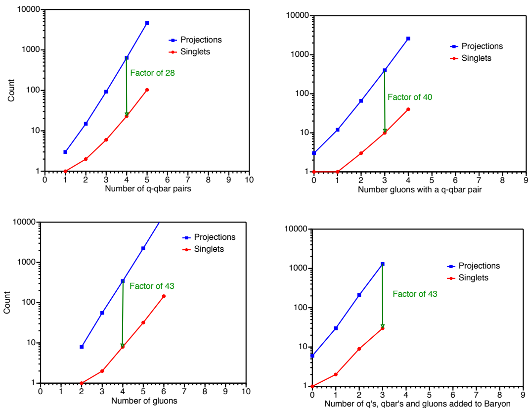
FIG. 12: (color online) Number of color space states that apply to each space-spin configuration of selected multi-parton states for two methods of enumerating the color basis states. The upper curves are counts of all color configurations with zero color projection. The lower curves are counts of global color singlets.
