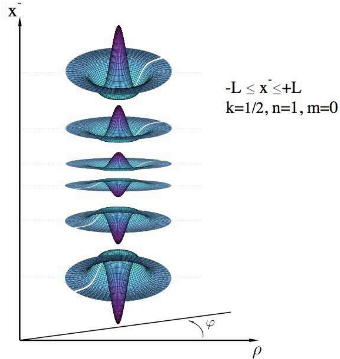
FIG. 4: (color online) Transverse sections of the real part of a 3-D basis function involving a 2-D harmonic oscillator and a longitudinal mode of Eq. 4 with antiperiodic boundary conditions (APBC). The quantum numbers for this basis function are given in the caption. The basis function is shown for the full range -L \leq x^- \leq L .
