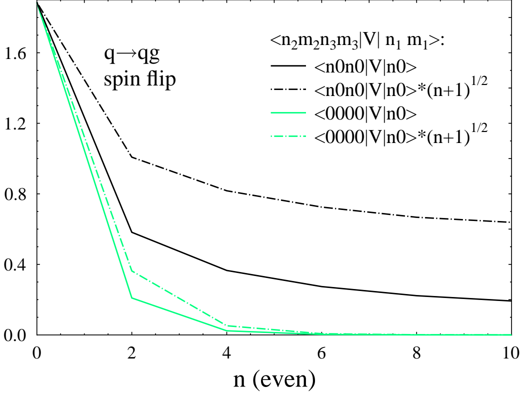
FIG. 13: (color online) Behavior of representative fermion to fermion-boson matrix elements in BLFQ. The quantum numbers specifying the parton transverse modes (n_i, m_i) in the matrix elements are given in the legend. Only the transverse mode contributions to the matrix elements are shown. Results are also shown with a multiplicative factor of \sqrt{n+1} applied to help search for a logarithmic divergence by obtaining a resulting flat behavior, when it occurs. Overall matrix element normalization depends on the specific values of light-front momentum fractions carried by the interacting partons.
