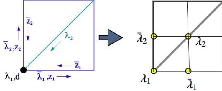
Figure 17: The fermions mapped onto a lattice with half the spacing can be recognized as reduced staggered fermions.
