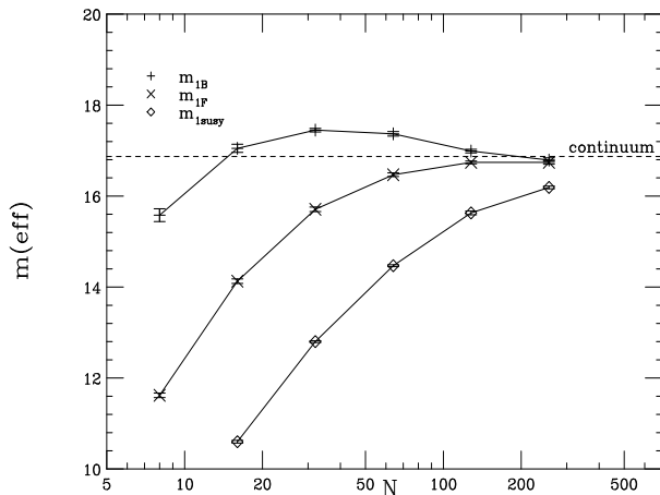
Figure 5: Counterterm corrected boson/fermion masses (From Giedt et al. [80])
