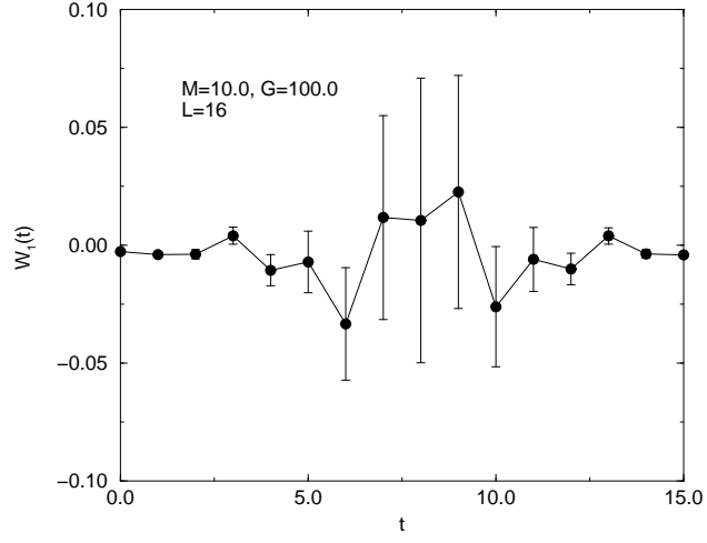
Figure 6: Ward identity for supersymmetric quantum mechanics
