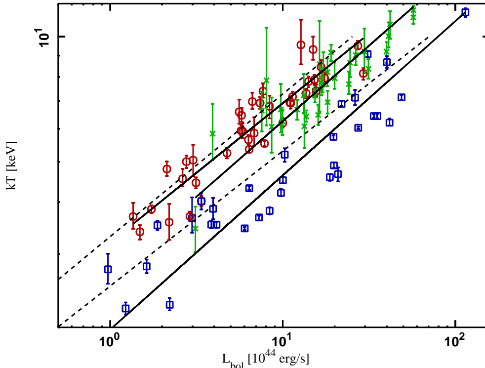
FIG. 12.— Luminosity temperature relation for low redshift clusters ( z < 0.2 , red circles), high redshift clusters ( z \geq 0.2 , green stars) and cooling core clusters (blue squares). Best fit L_X - T relations are shown as solid lines and the non-cooling and cooling samples at z = 0 of Allen & Fabian (1998) are shown as dashed lines.
