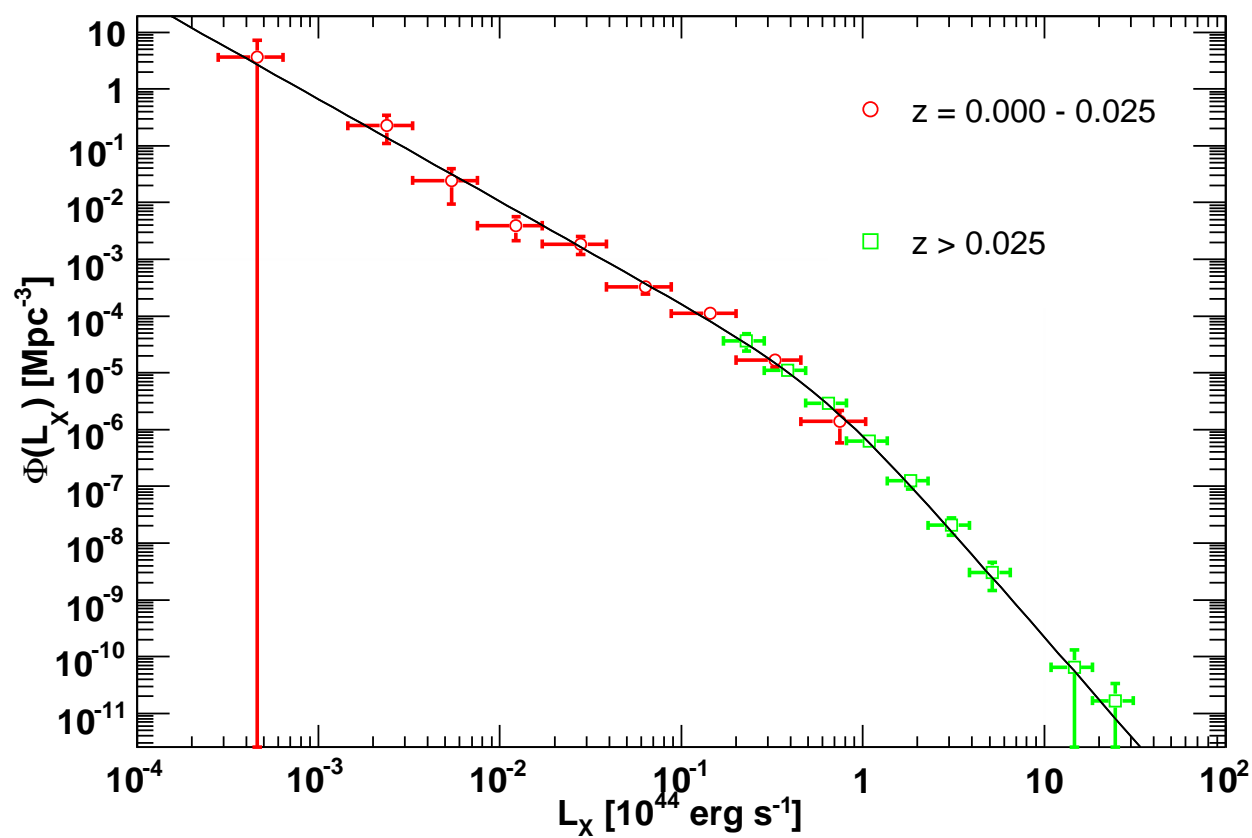
Fig. 6.— Luminosity function of the Seyfert-like AGNs, derived using the 1/V_{MAX} method, in two redshift bins (data points). The solid line is a non-evolving XLF double power-law model (model 1 in Tab. 4) as derived from the ML algorithm.
