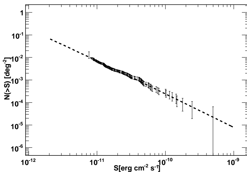
Fig. 5.— Cumulative \log N - \log S of the BAT Seyferts. The dashed line is the prediction of the best-fit XLF (model 1 in Tab 4).
