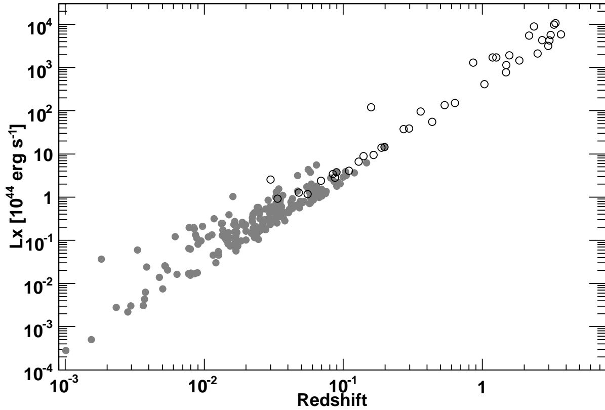
Fig. 3.— Luminosity-redshift plane for the BAT blazars (empty circles) and BAT Seyfert-like AGNs (filled gray circles).
