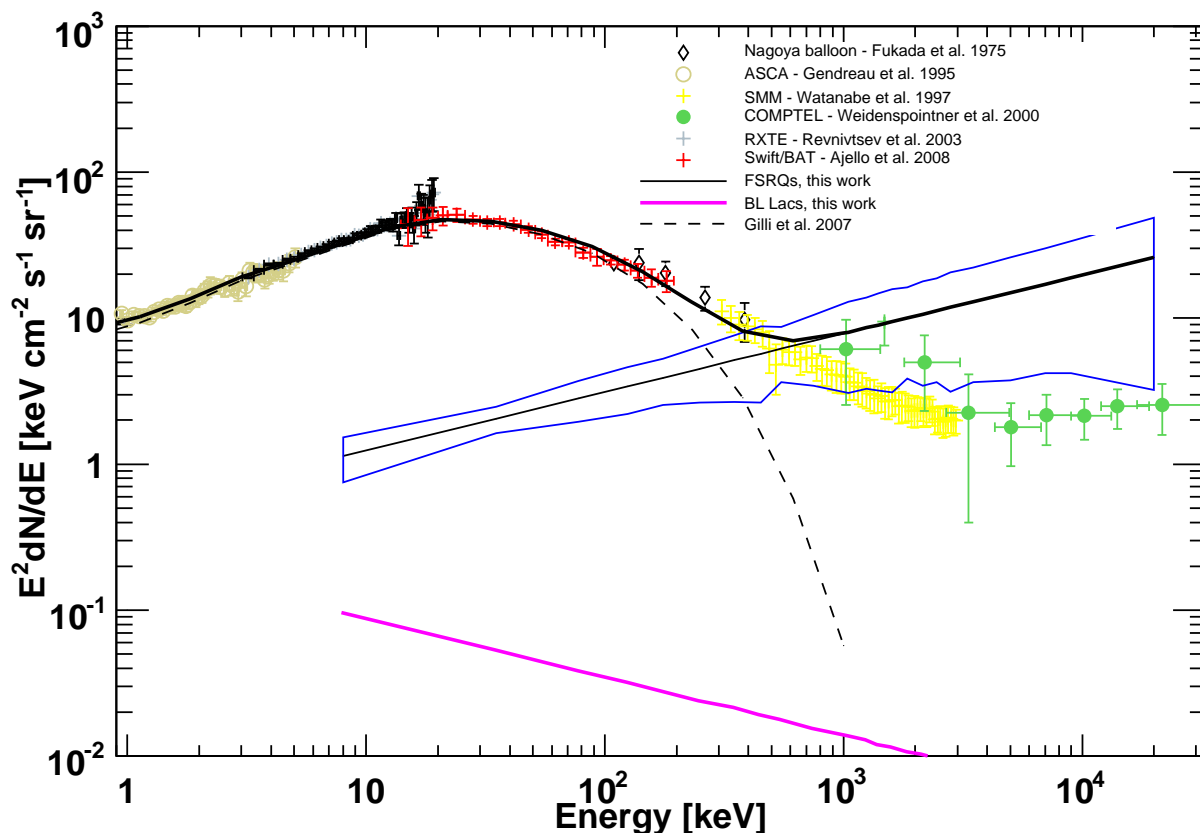
Fig. 15.— Spectrum of the CXB and contribution of the FSRQs (blue region). The data points are different measurements of the diffuse background as indicated in the label (Fukada et al. 1975; Gendreau et al. 1995; Watanabe et al. 1997; Weidenspointner et al. 2000; Revnivtsev et al. 2003; Ajello et al. 2008b). The dashed line is the total contribution of Seyfert-like AGNs computed with the model of Gilli et al. (2007) arbitrarily multiplied by 1.1 to fit the CXB emission at 30 keV. The solid line is the sum of the Seyfert-like and FSRQs. The spectrum of FSRQs has been modeled as a power-law with a mean photon index of 1.6. The blue region represents the range of values obtained from the Monte Carlo realizations of best-fit parameter ranges. The magenta solid line represents the contribution of BL Lac objects whose uncertainty is not plotted for clarity, but is, due to the low number of objects, > 30\% at any energy.
