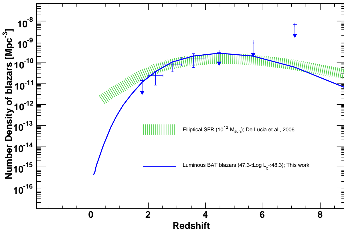
Fig. 18.— Density of the most luminous BAT blazars ( 47.3 < \text{Log } L_X < 48.3 , blue datapoints and line) compared to the prediction of the evolution of massive elliptical galaxies of De Lucia et al. (2006). The curve of De Lucia et al. (2006) was rescaled to match the BAT luminosity function. In order to consider also the contribution of misaligned jets, the space density of blazars (y-axis) needs to be multiplied by a factor in the 200-800 range (see § 6 for details).
