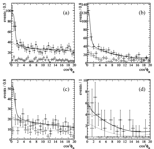
FIG. 1: Distributions of \cos^2\phi_B for B^0 \rightarrow \pi^-\ell^+\nu_\ell (a), B^+ \rightarrow \pi^0\ell^+\nu_\ell (b), B^+ \rightarrow \eta\ell^+\nu_\ell (c) and B^+ \rightarrow \eta'\ell^+\nu_\ell (d) candidates; filled and hollow circles represent D mass peak and sideband data, respectively. The curves are stacked fit results for “cmb” (dotted), “bg” (dashed) and “sig” (solid) PDFs, as defined in the text. The fits are performed in bins of q^2 but are here shown in the full q^2 range.
