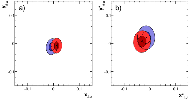
FIG. 11: (color online). Contours at 39.3% (dark) and 86.5% (light) 2-dimensional confidence-level (CL) in the (a) (x_{\mp,\pi}, y_{\mp,\pi}) and (b) (x_{\mp,\pi}^*, y_{\mp,\pi}^*) planes, corresponding to one- and two-standard deviation regions (statistical only), for B^- \rightarrow D^{(*)0} \pi^- (thick and solid lines) and B^+ \rightarrow \bar{D}^{(*)0} \pi^+ (thin and dotted lines) control sample decays. Note the differences in scale when comparing to Figs. 9 and 10.
