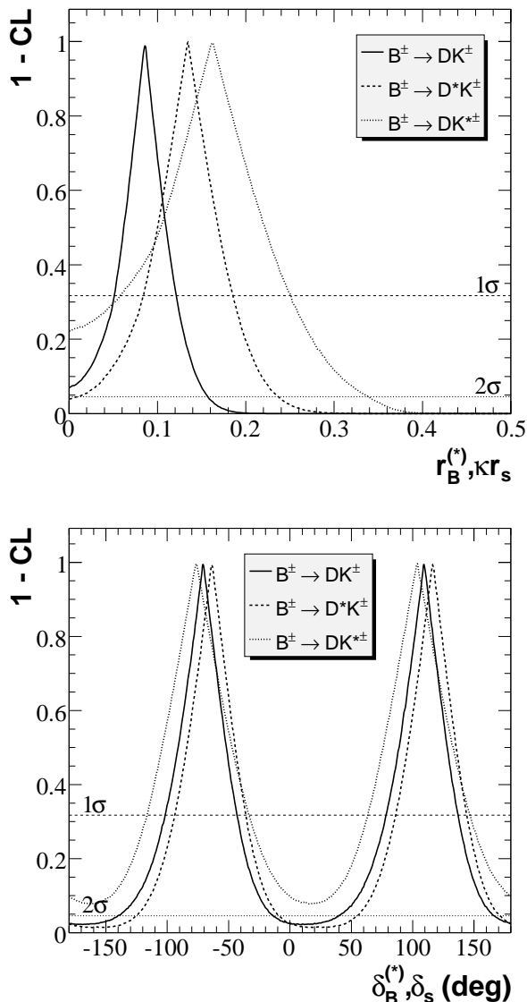
FIG. 13: \alpha = 1 - \text{CL} as a function of (a) r_B , r_B^* , and \kappa r_s , and (b) \delta_B , \delta_B^* , and \delta_s , for B^- \rightarrow \tilde{D}^0 K^- , B^- \rightarrow \tilde{D}^{*0} K^- , and B^- \rightarrow \tilde{D}^0 K^{*-} decays, including statistical and systematic uncertainties and their correlations. The dashed (upper) and dotted (lower) horizontal lines correspond to the one- and two-standard deviation intervals, respectively.
