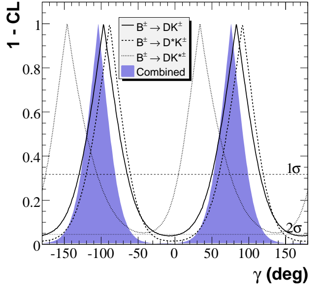
FIG. 12: (color online). \alpha = 1 - \text{CL} as a function of \gamma for B^- \rightarrow \tilde{D}^0 K^- , B^- \rightarrow \tilde{D}^{*0} K^- , and B^- \rightarrow \tilde{D}^0 K^{*-} decays separately, and their combination, including statistical and systematic uncertainties and their correlations. The dashed (upper) and dotted (lower) horizontal lines correspond to the one- and two-standard deviation intervals, respectively.
