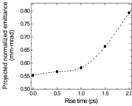
Figure 7: Norm. rms emittance versus rise time.
