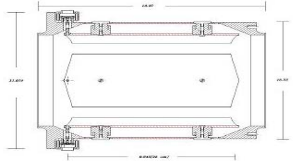
Figure 3: Floating-ground BPM for the SNS ring.
