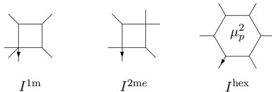
FIG. 2: The three independent integrals which contribute to the six-particle amplitude at one loop. The external momenta are labeled clockwise, beginning with k_1 which is denoted by an arrow. The \mu_p^2 in the hexagon integral indicates that a factor of the square of the (-2\epsilon) -dimensional components of the loop momentum is to be inserted in the numerator of the integrand.
