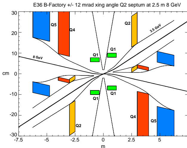
Figure 11. Layout of a preliminary design for the IR of a 1 \times 10^{36} \text{cm}^{-2} \text{sec}^{-1} luminosity machine at SLAC. There are no dipole magnets to bring the beams into collision. Instead a crossing angle of \pm 12 mrad is used. The shared quadrupoles are superconducting and are symmetrically positioned to generate the same bending in the beam
