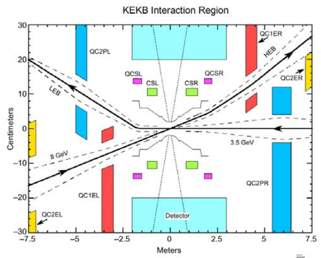
Figure 7. Layout of the KEKB IR. The incoming beams are on-axis and the outgoing beams are off-axis in the shared QC1EL and QC2EL superconducting quadrupoles. Note the expanded vertical scale. For comparison, the scales in this plot are the same as the scales used for the PEP-II layout in Figure 1.
