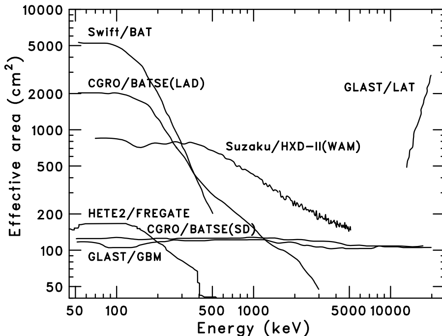
Fig. 10. Comparison of the effective area of the anti-counter units per side (excluding the “Corner Units”) and those of other GRB detectors.
