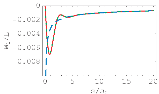
Figure 1: (Color) Plot of the wake function per unit length W_1(s)/L as a function of s/s_0 . The solid(red) curve stands for the full wake, the dashed(blue) curve for the long-range wake, and the dotted(green) curve for the numerical results with all three terms in the denominator of Eq. (4).
