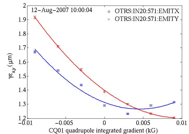
Figure 9: Horizontal (blue) and vertical (red) emittance at 135 MeV and 1 nC optimized (parabolic fit) by varying the gun-solenoid’s ‘normal’ quadrupole coil field, CQ01 .
