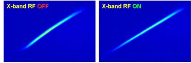
Figure 36: Beam on the BC1 OTR screen with its large horizontal dispersion. The LIS RF phase is off crest by 25°. The first RF deflector is ‘ON’, and the X-band cavity is ‘OFF’ at left, and ‘ON’ (20 MV) at right, demonstrating proper X-band linearization of the energy chirp.
