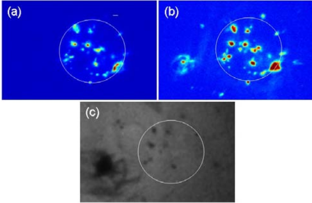
Figure 12: Electron emission images on a YAG screen 1.4 m from the cathode, (a) and (b), taken on June 23, and images of the cathode taken using a white light source and camera, (c), taken on June 20. Image (a) is taken with the laser iris set for a 1.3-mm spot diameter and image (b) is taken with the iris fully open. The circle outlines the nominal 1.3-mm diameter laser illumination area.
