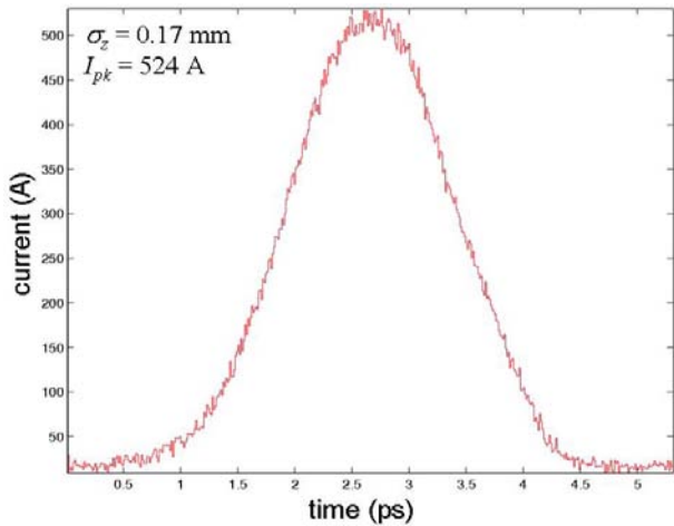
Figure 38: Bunch length distribution measured using both RF deflectors. The first measurement is at 135 MeV (top: \sigma_z \approx 1.1 mm, I_{pk} \approx 97 A) and the second is at 14 GeV (bottom: \sigma_z \approx 0.17 mm, I_{pk} \approx 520 A), representing the bunch length before and after BC1 compression at 1 nC.
