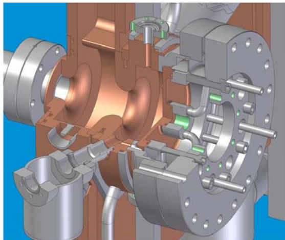
Figure 6: The LCLS gun in cut-away view showing the full and half cells with the cathode flange at right.
