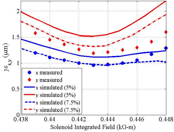
Figure 34: Measured and simulated emittance vs. gun-solenoid field. The measured emittances use a 5% area-cut, while simulations are shown for 5% and 7.5%.
