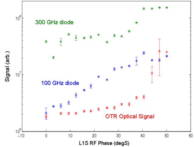
Figure 41: The signals of the BL12 microwave detectors at 100 GHz (blue) and 300 GHz (green), and the image-integrated OTR optical signal (red), as seen by a digital camera, are plotted (log-scale) as functions of the L1S RF phase relative to the accelerating crest (at phase = 0). The increase in the OTR signal suggests the on-set of COTR.
