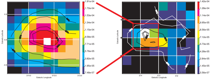
Fig. 3 Likelihood test statistics map of the region of the Kookaburra complex between 2 and 4 GeV. The source location is at (l=313.71, b=0.04) , close to the previously reported location of 3EG J1420–607 at (l=313.63, b=0.37) , but not confirming the location at GEV J1417–6100 at (l=313.18, b=0.14) . The EGRET source indeed coincides with HESS J1420–607. There is substantial excess emission towards HESS J1418–609, though.
