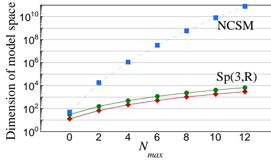
Figure 1. Dimension of the NCSM (blue squares) and J = 0, 2 , and 4 \text{Sp}(3, \mathbb{R}) (red diamonds for the 3 most significant 0p-0h irrep case and green circles for when all 13 0p-0h irreps are included) model spaces as a function of maximum allowed \hbar\Omega excitations, N_{max} .
