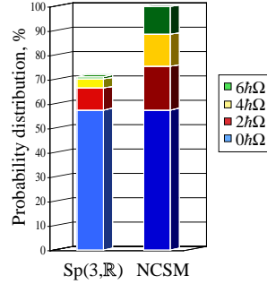
Figure 3. ^{16}\text{O} ground 0^+ state probability distribution over 0\hbar\Omega (blue, lowest) to 6\hbar\Omega (green, highest) subspaces for the leading 0p-0h ( 0\ 0 ) \text{Sp}(3, \mathbb{R}) irrep case (left) and NCSM (right) for N_{max} = 6 and bare JISP16 interaction.
