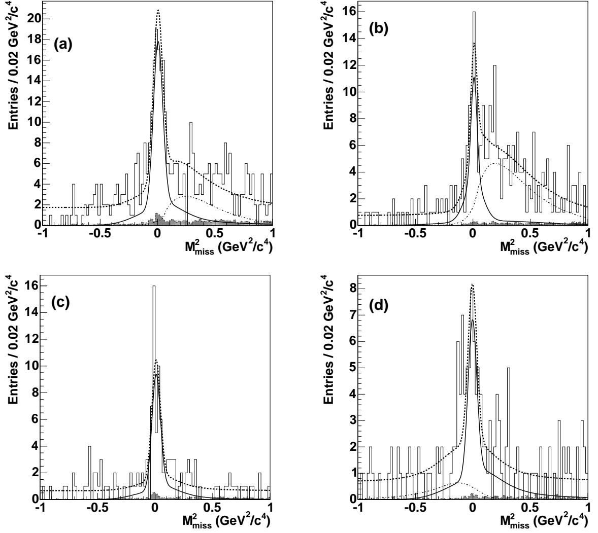
Figure 14: Missing mass against D^* \pi in full recoil tagged events. The modes considered are (a) D^+ \pi^- l^- \bar{\nu} , (b) D^0 \pi^+ l^- \bar{\nu} , (c) D^{*+} \pi^- l^- \bar{\nu} and (d) D^{*0} \pi l^- \bar{\nu} .
