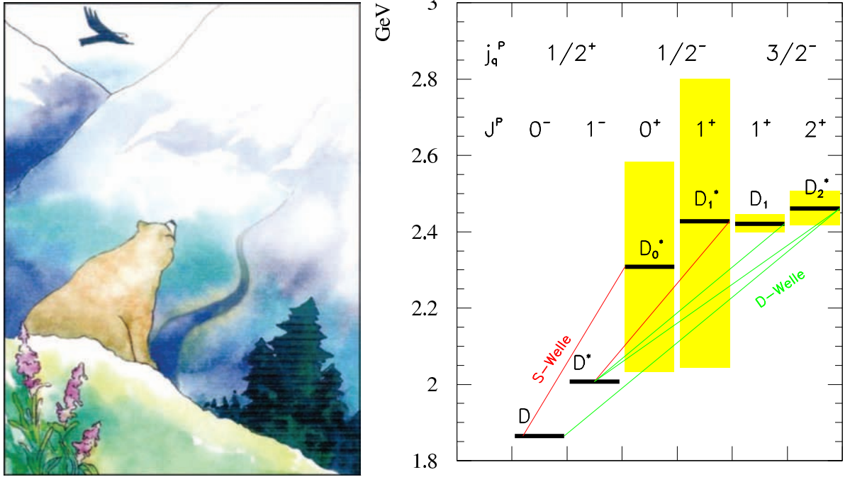
Figure 10: “...to see what he could see...and high mass charm states we might see...” [13]
