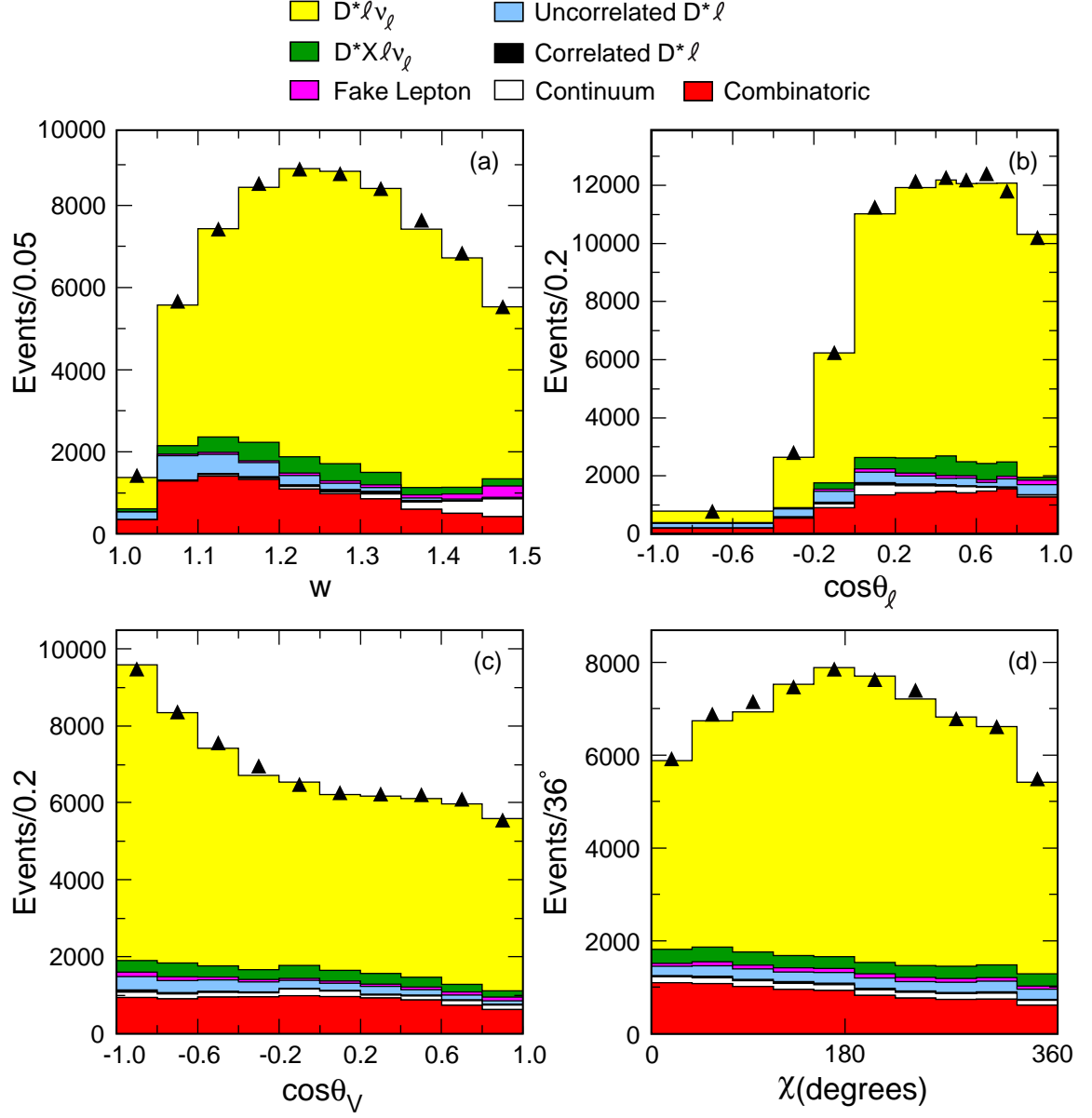
Figure 7: Projection results for w , \cos\theta_\ell , \cos\theta_V . The angle \chi was not part of the fit.
