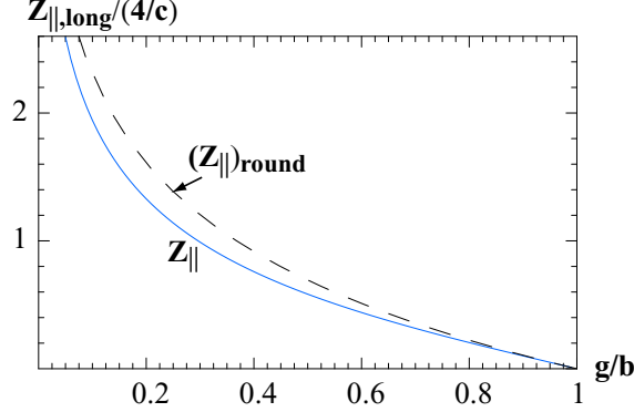
FIG. 10: For a thin flat iris with aperture 2g in a flat beam pipe of aperture 2b , the longitudinal impedance Z_{\parallel, long} as function of \alpha = g/b . The round case, (Z_{\parallel})_{round} = 4 \ln(b/g)/c , is also shown (dashes).
