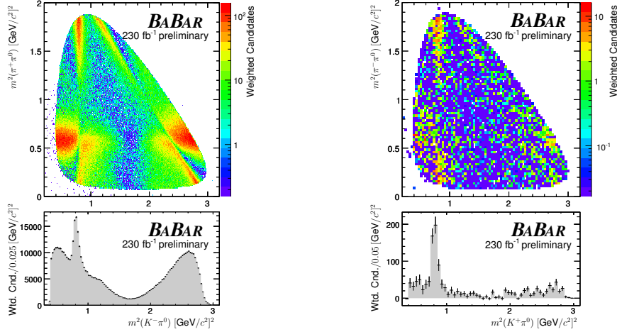
Fig. 2. Dalitz plot and one-dimensional projection onto m_{K\pi^0}^2 for the CF decay (left) and the DCS decay (right). A statistical background subtraction has been applied ( i.e. candidates have been weighted), and distributions have been corrected for efficiency variations as a function of the Dalitz plot. The shaded histograms in the lower plots are projections of the Dalitz plots above them, with error bars superimposed. Candidates have been selected requiring the event-level tag.
