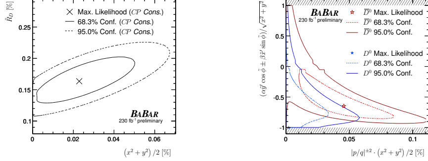
Fig. 3. Contours of constant \Delta \ln \mathcal{L} = 1.15, 3.0 in terms of the doubly Cabibbo-suppressed rate and the integrated mixing rate (left). The upward slope of the contour indicates negative interference. Contours of constant \Delta \ln \mathcal{L} = 1.15, 3.0 in terms of the normalized interference term and the integrated mixing rate, for the D^0 and \bar{D}^0 samples separately (right). The hatched regions are physically forbidden.
