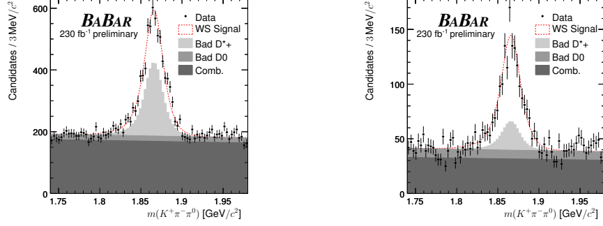
Fig. 1. The m_{K\pi\pi^0} distribution with fitted PDFs overlaid for the WS data sample used to search for D mixing (left) and for the sample used to obtain the Dalitz-plot distributions (right). The sample on the right requires a second, event-level, flavor tag. Both distributions require 0.1444 < \Delta m < 0.1464 \text{GeV}/c^2 .
