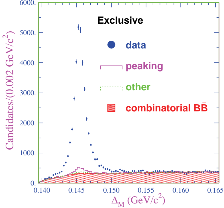
Figure 2: The \Delta_M mass distribution of the exclusive sample, after continuum subtraction. The data are represented by points with its error. The hatched histogram shows the combinatorial B\bar{B} background. The other histograms show the uncorrelated peaking (solid histogram) and Cabibbo suppressed decays or other (dotted histogram), respectively.
