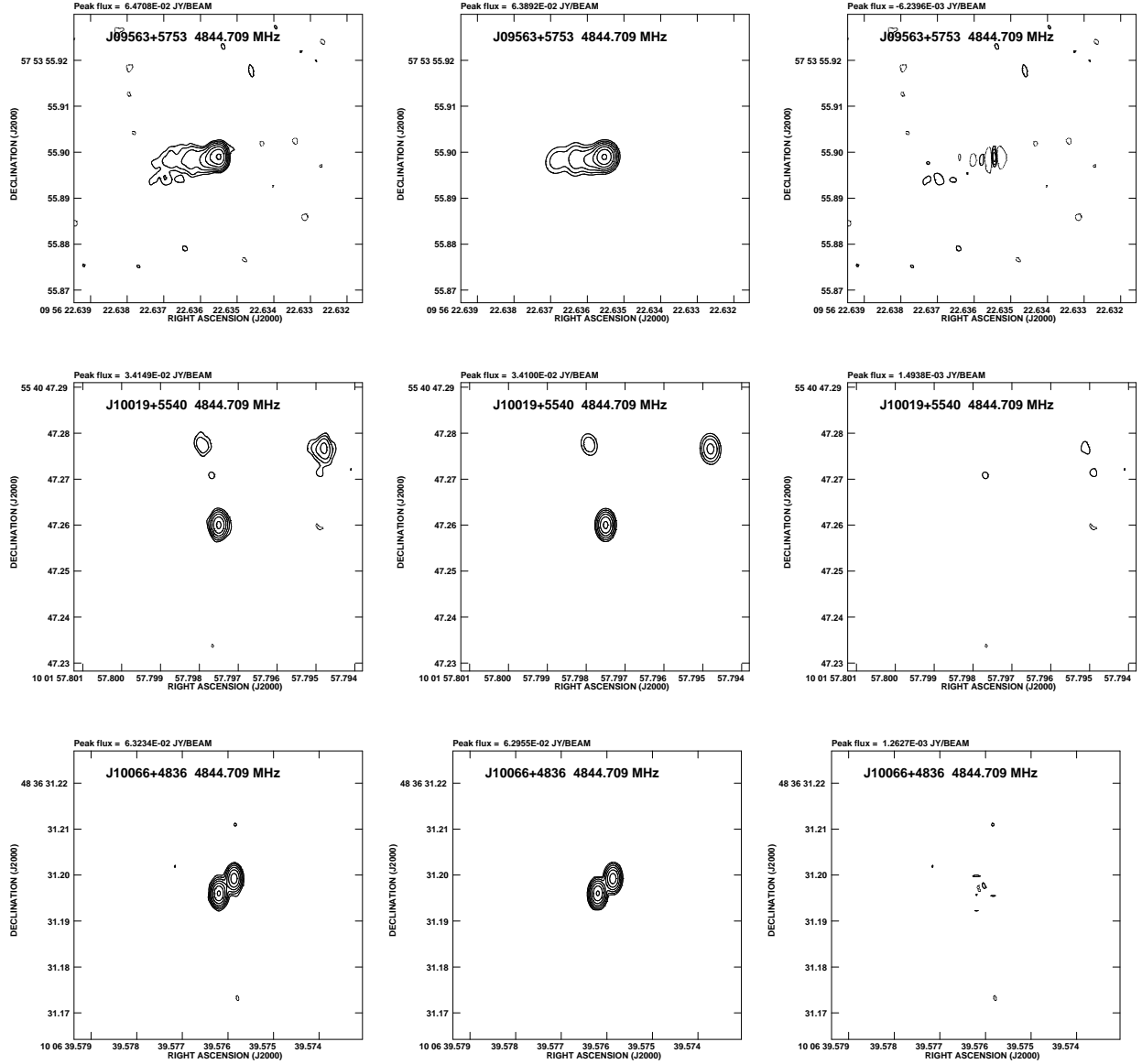
Fig. 3.— For three VIPS sources, the 5 GHz I maps (left column), the Gaussian fits to the I maps (middle column), and the residuals for the Gaussian component fits (right column) for a core-jet system (upper panels), a complex system (middle panels), and a CSO candidate (lower panels).
