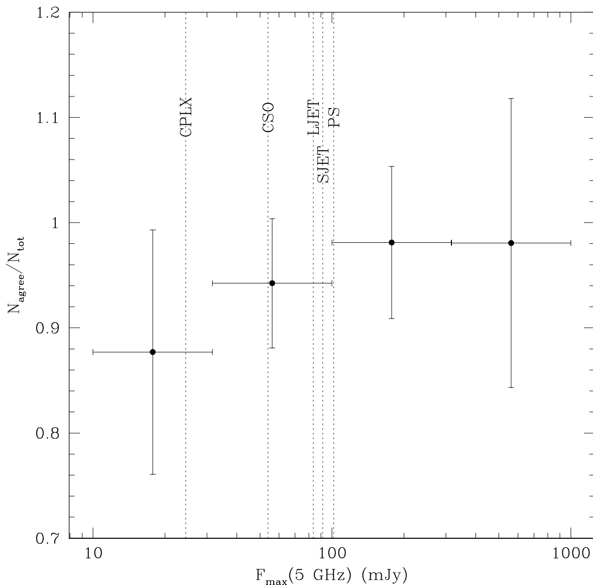
Fig. 5.— Within bins of peak 5 GHz flux density, the fraction of sources for which the “bye-eye” classification agrees with the automatic classification algorithm (see §2.3). The median peak 5 GHz flux densities for the five sources categories are displayed as vertical dotted lines.
