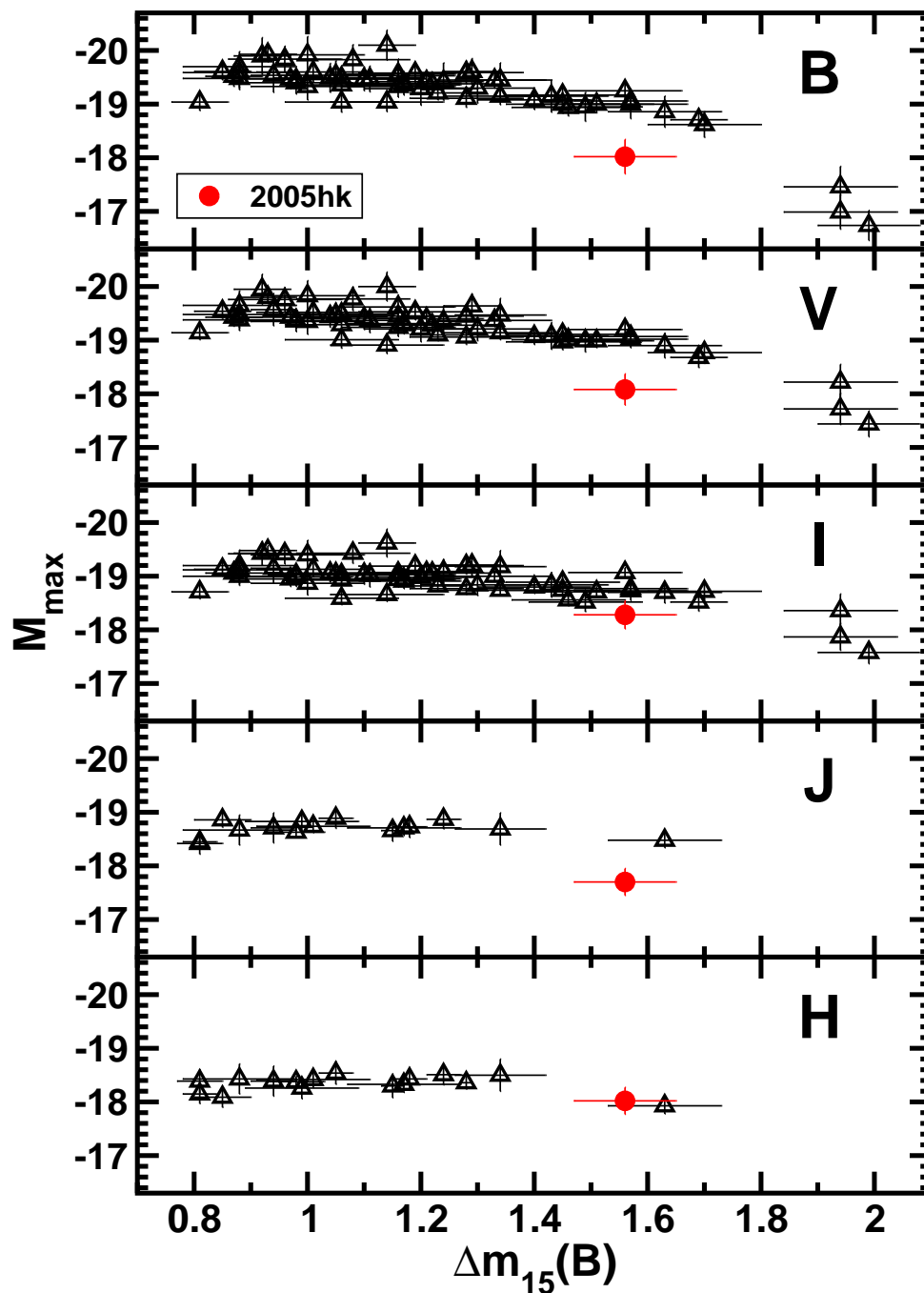
Fig. 14.— The absolute magnitudes of SNe Ia at maximum light in the BVIJH bands plotted versus the decline rate parameter \Delta m_{15}(B) . The black triangles are SNe in the redshift range 0.01 < z < 0.1 whose distances were calculated from their host galaxy radial velocities in the cosmic microwave background frame assuming a Hubble constant of H_0 = 72 \text{ km s}^{-1} \text{ Mpc}^{-1} . The red circle in each panel corresponds to SN 2005hk.
