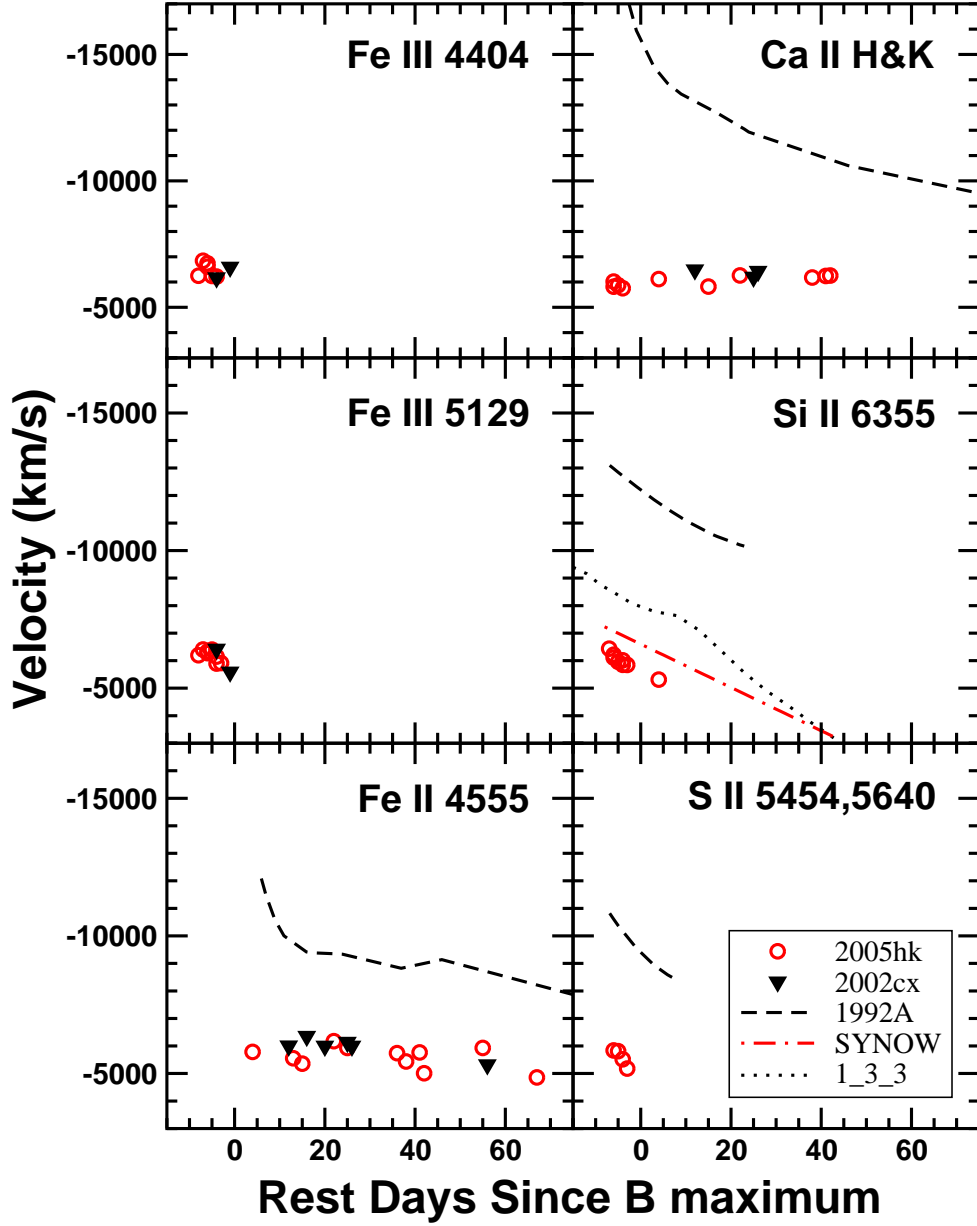
Fig. 9.— Expansion velocities for SN 2005hk (circles) and SN 2002cx (triangles) in selected lines of Fe II, Fe III, Ca II, Si II, and S II. The measurements were estimated from the wavelength of the minimum of each feature, correcting for the heliocentric velocities of the host galaxies. For comparison, measurements in the Fe II, Ca II, Si II, and S II lines are shown for SN 1992A, a typical SN Ia with a decline rate of \Delta m_{15}(B) = 1.47 . The evolution of the photospheric velocity of SN 2005hk as estimated from SYNOW fits is compared with the Si II \lambda 6355 measurements. Finally, in the same plot, the velocity of the “Rosseland” photosphere for the 3D deflagration model 1_3_3 is indicated.
