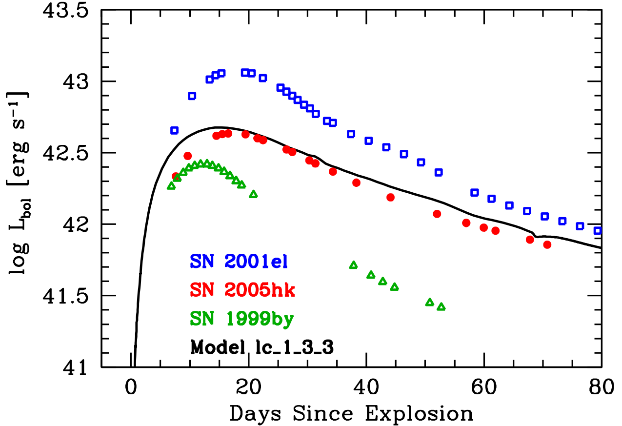
Fig. 15.— UVOIR bolometric light curve of SN 2005hk plotted with respect to the epoch of explosion. For reference, the UVOIR light curves of SN 2001el ( \Delta m_{15}(B) = 1.13 ) and SN 1999by ( \Delta m_{15}(B) = 1.90 ) are also plotted as blue squares and green triangles, respectively. For SN 2005hk, the explosion is assumed to have occurred 17 days before B maximum, whereas for SN 2001el and SN 1999by this number is taken to be 18.1 and 11.0 days before B maximum, respectively. The data for SN 2005hk are compared with the UVOIR light curve for the 3D deflagration model lc_1_3_3 . See text for further details.
