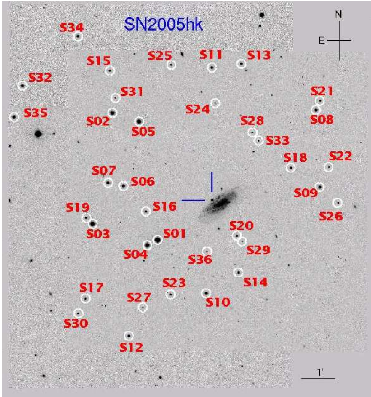
Fig. 1.— The field of SN 2005hk observed with the Swope 1-m telescope at LCO. This image was created by combining optical and infrared images so that some of the stars used for the NIR photometry would be clearer. North is up and East is to the left. The supernova is marked to the NE of the host galaxy nucleus. The comparison stars used to derive differential photometry of the SN are labeled. The plate scale is shown near the bottom right.
