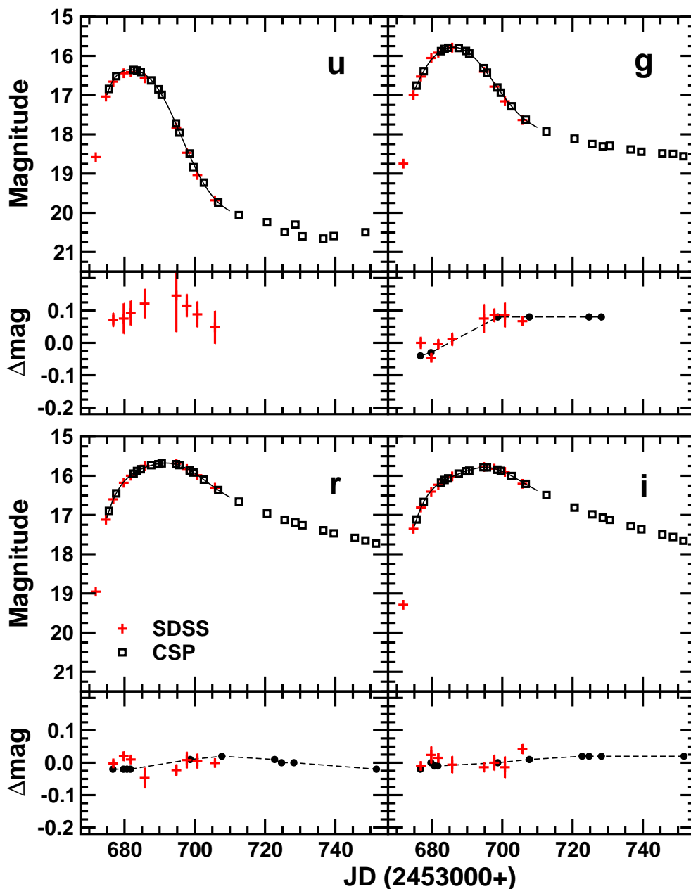
Fig. 7.— Comparison of observed ugri light curves of SN 2005hk obtained by the CSP and SDSS II. In the top panels for each filter, the square symbols correspond to the CSP measurements and the crosses to SDSS II. The solid line represents a fit to the CSP data. In the lower panels, the difference between the SDSS II magnitudes and the smooth fit to the CSP data is shown. These differences compare well with the S corrections (indicated by the solid circles joined by dashed lines) calculated via synthetic photometry from the respective response functions of the CSP and SDSS II passbands.
