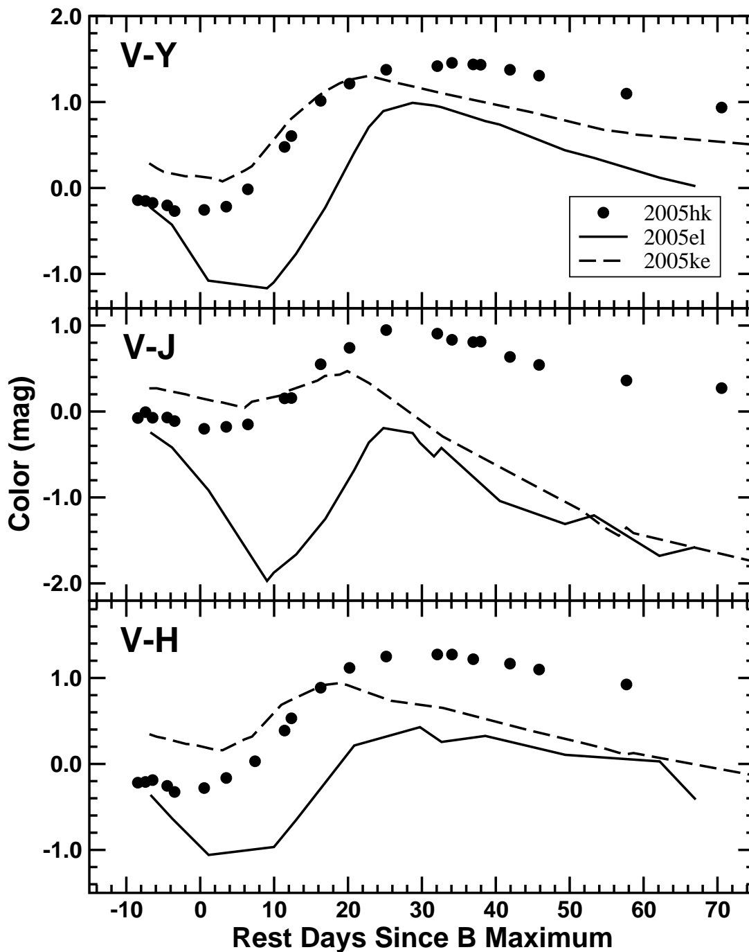
Fig. 13.— Comparison of the V - Y , V - J , and V - H color evolution of SN 2005hk with CSP observations of SN 2005el ( \Delta m_{15}(B) = 1.47 ) and SN 2005ke ( \Delta m_{15}(B) = 1.82 ). The colors have been corrected for Galactic extinction using the estimates of Schlegel, Finkbeiner, & Davis (1998).
