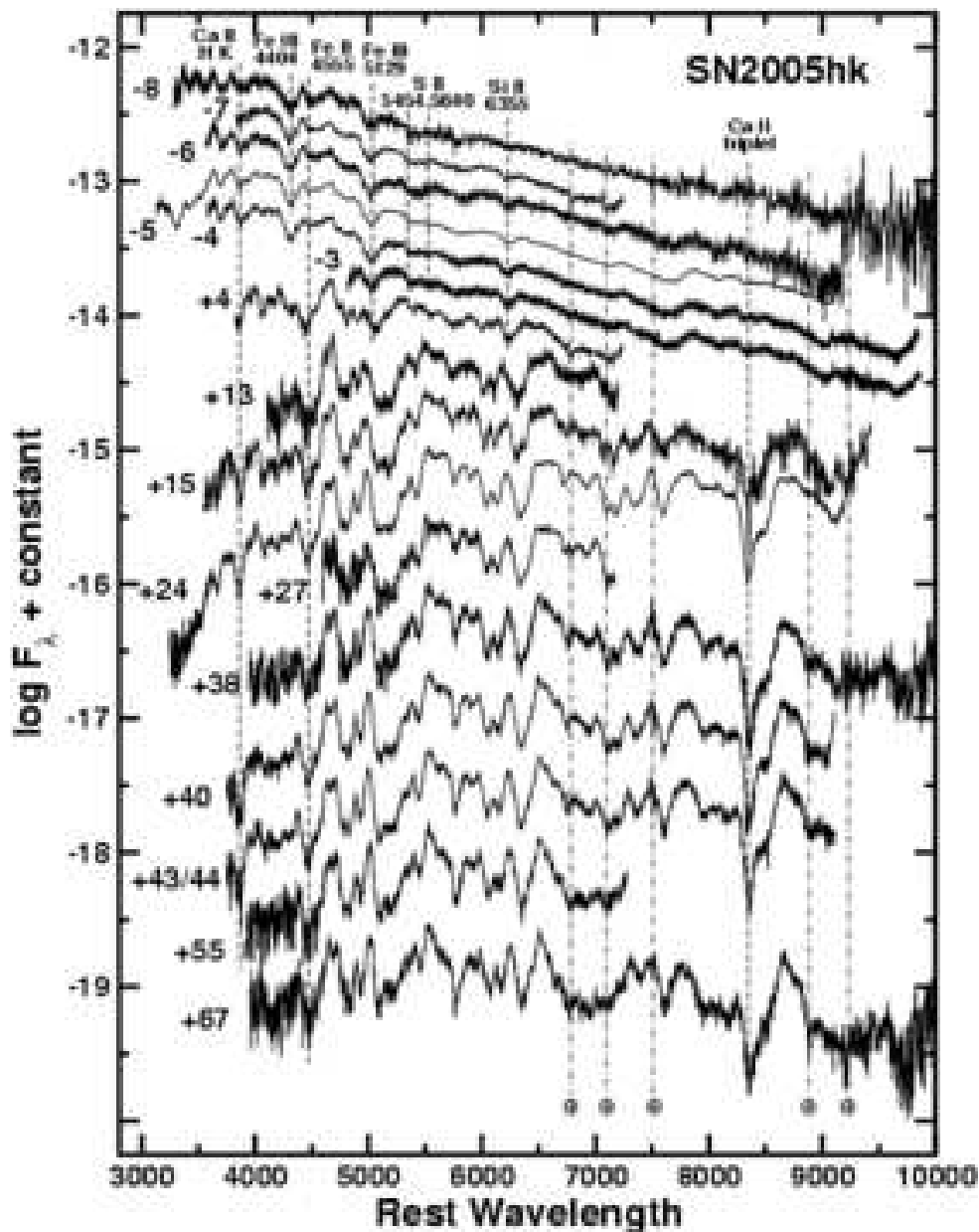
Fig. 2.— Spectroscopic evolution of SN 2005hk. Each spectrum is plotted on a logarithmic flux density scale, shifted by an arbitrary constant. The wavelengths of the spectra were shifted to the SN rest frame using a redshift of z = 0.012993 as given in NED. The labels to the left of each spectrum indicate the epoch in rest-frame days since the date of B maximum ( JD = 2,453,685.1 ). The spectra for days +43 and +44 have been averaged. Identifications for selected spectral features are indicated. For most (but not all) of the spectra, the telluric absorption features have been eliminated; the positions of the strongest of these are indicated by the \oplus symbol.
