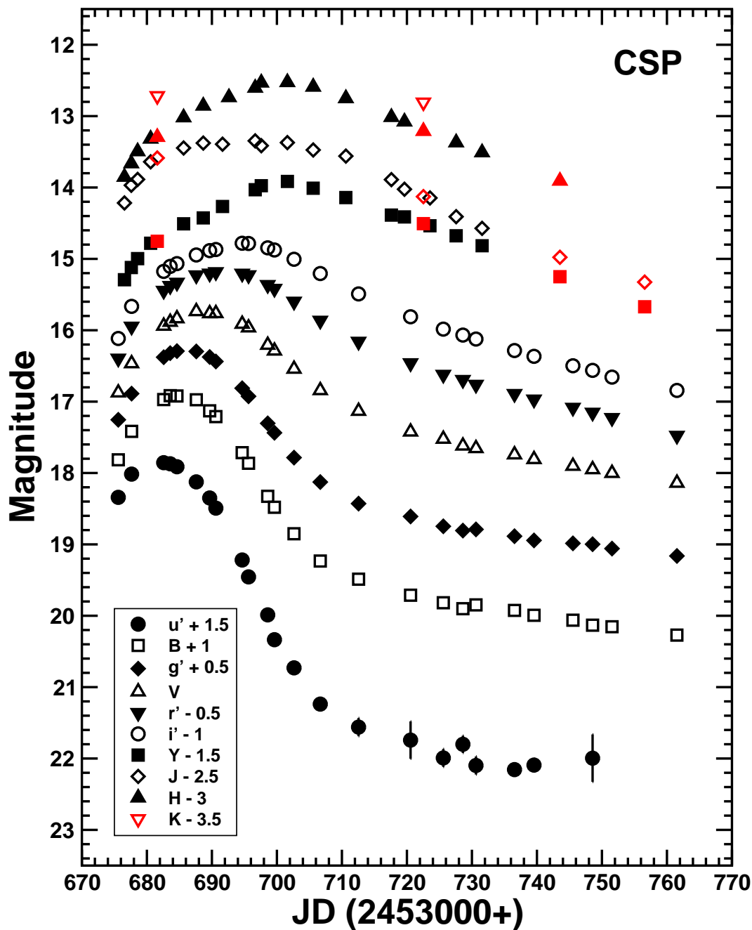
Fig. 4.— Observed u'g'r'i'BV and YJHK light curves of SN 2005hk obtained by the CSP. For clarity, the magnitudes in each band have been shifted by an arbitrary constant which is given in the legend. The errors in the measurements are smaller than the plot symbols except where indicated. YJH photometry obtained with RetroCam is plotted with black symbols; YJHK measurements made with WIRC are shown in red.
