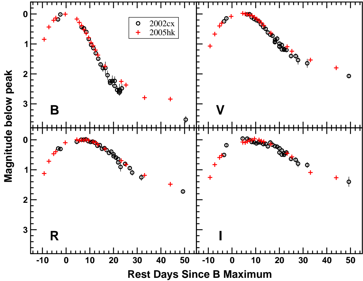
Fig. 10.— Comparison of KAIT BVRI photometry of SN 2005hk (red plus symbols) and SN 2002cx (black circles). The light curves have been normalized to the same peak magnitudes.
