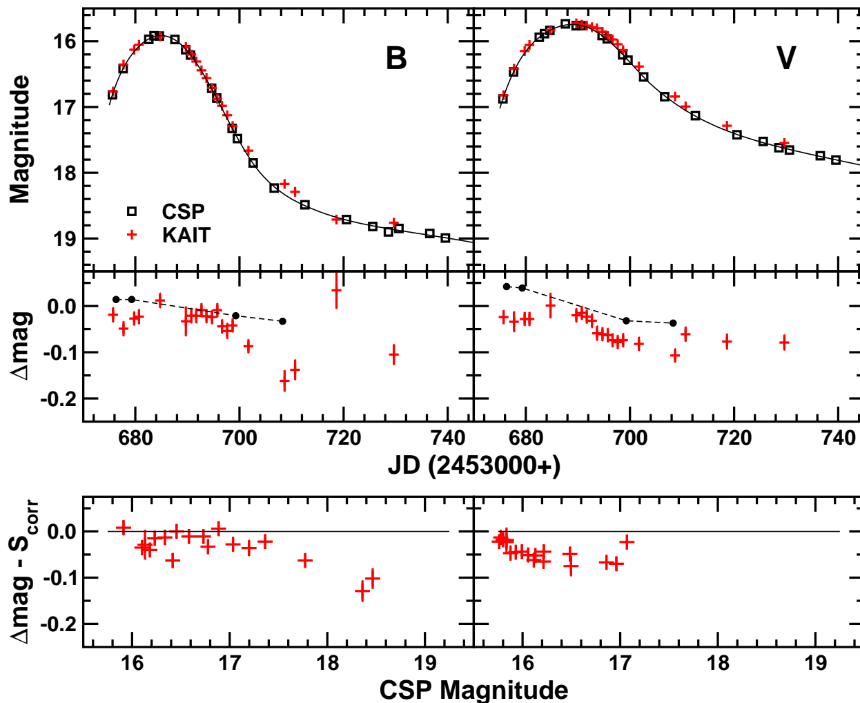
Fig. 6.— Comparison of observed BV light curves of SN 2005hk obtained by the CSP and KAIT. In the top panels, the square symbols correspond to the CSP measurements and the crosses to KAIT. The solid line represents a fit to the CSP data. In the middle panels, the difference between the KAIT magnitudes and the smooth fit to the CSP data is shown. Also indicated by the solid circles joined by dashed lines are the expected S corrections calculated via synthetic photometry with the respective response functions of the CSP and KAIT passbands. (See text for more details). In the lower panels, the S corrections have been subtracted from the magnitude differences between the KAIT and CSP measurements and then plotted vs. the CSP magnitude.
