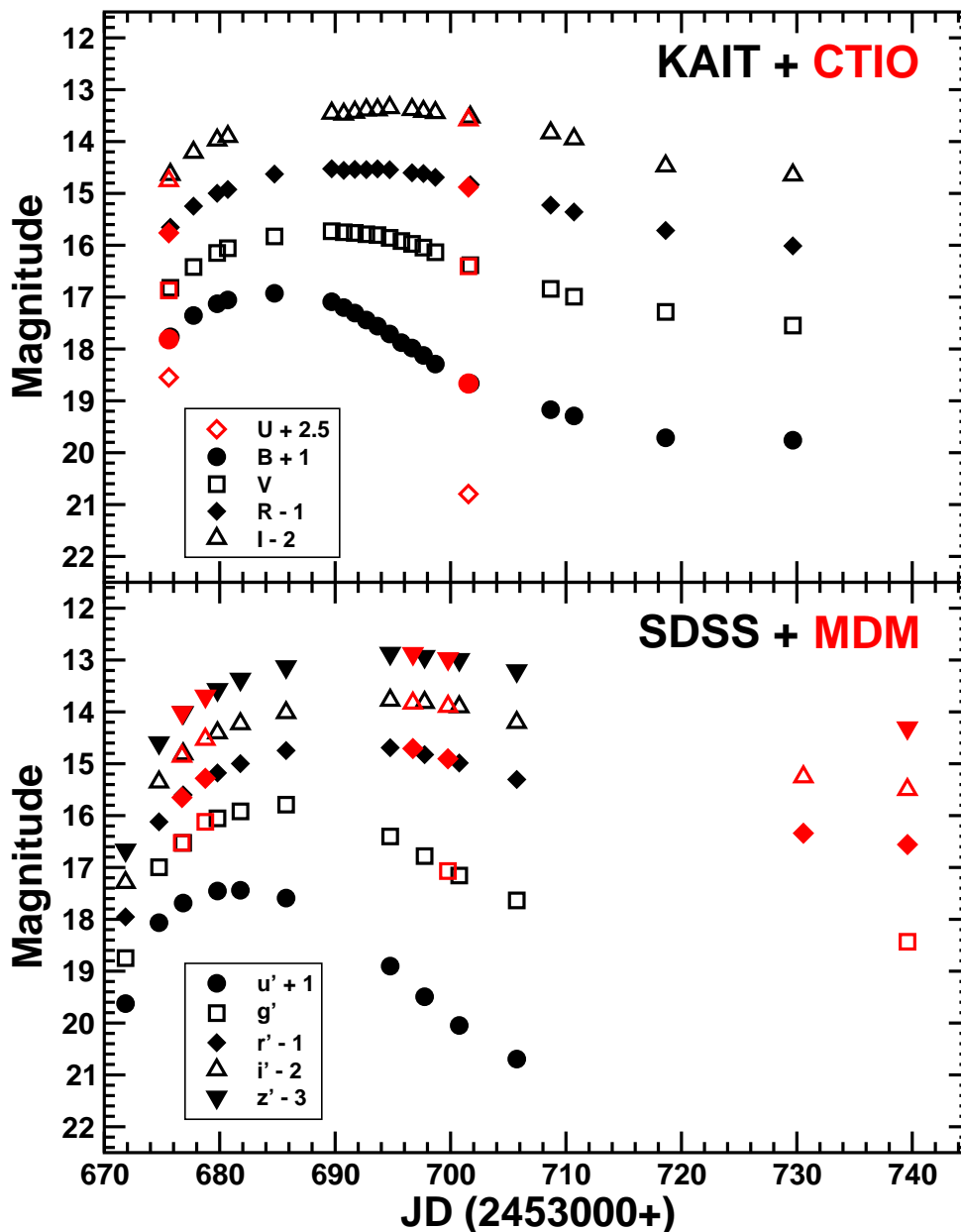
Fig. 5.— (Above) Observed BVRI light curves of SN 2005hk obtained by KAIT and with the CTIO 0.9 m. The KAIT data are plotted with black symbols, and the CTIO with red. Error bars are not shown as these are considerably smaller than the plot symbols. No host galaxy subtraction was performed on the images before measurement. (Below) Observed ugriz light curves of SN 2005hk obtained by the SDSS II Supernova Survey. The SDSS and MDM photometry is derived from the scene modeling algorithm of Holtzman et al. (2007). Error bars are much smaller than the plot symbols.
