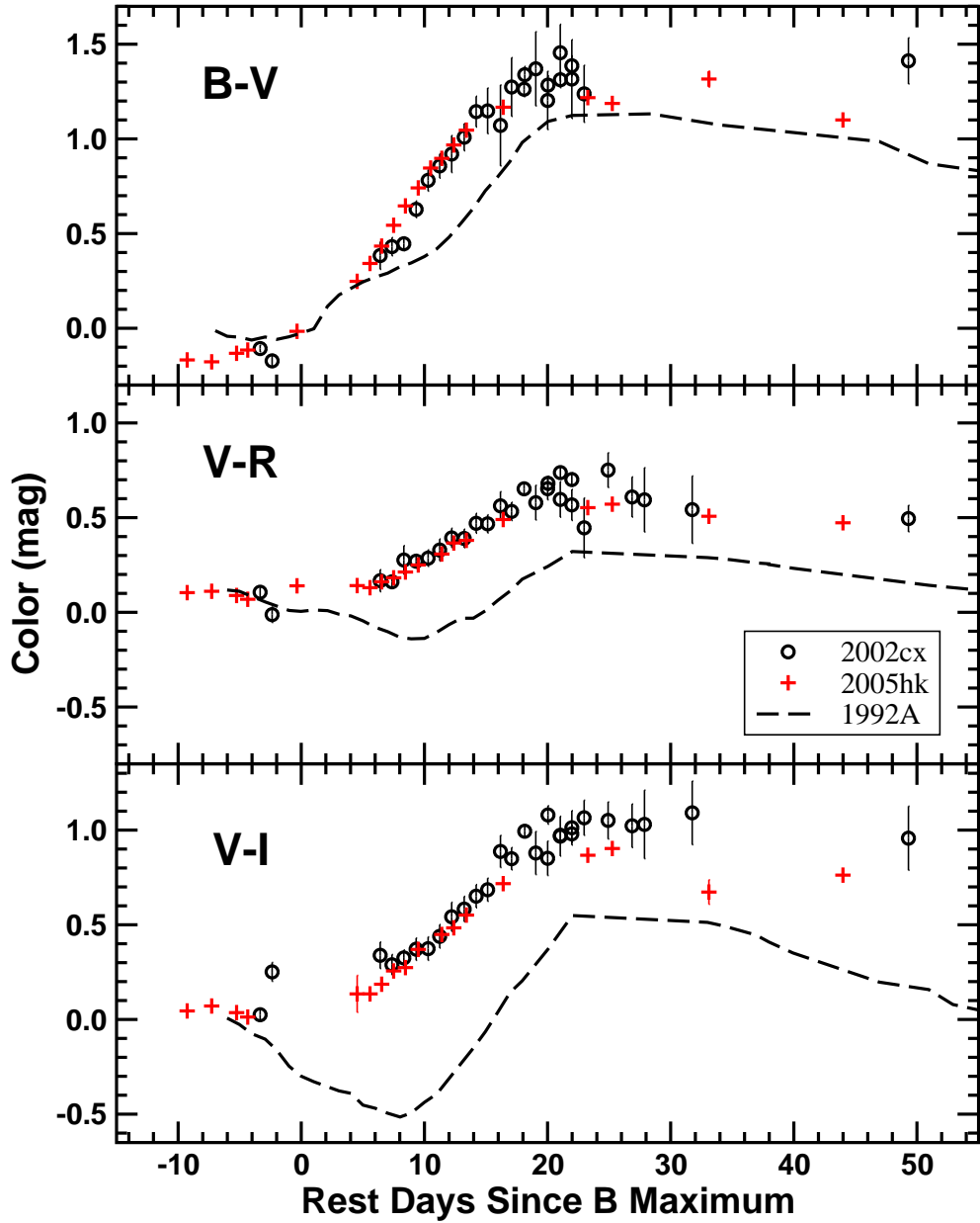
Fig. 11.— Comparison of the B-V , V-R , and V-I color evolution of SN 2005hk (red plus symbols) and SN 2002cx (black circles) as derived from KAIT photometry. The colors have been corrected for Galactic extinction assuming the Schlegel, Finkbeiner, & Davis (1998) estimates of E(B-V)_{\text{Gal}} = 0.022 for SN 2002hk and 0.034 for SN 2002cx. The colors of SN 2005hk have also been corrected for a host galaxy extinction of E(B-V)_{\text{Host}} = 0.09 . The color evolution of SN 1992A, a typical unreddened SN Ia with a decline rate of \Delta m_{15}(B) = 1.47 , is indicated by the dashed line.
