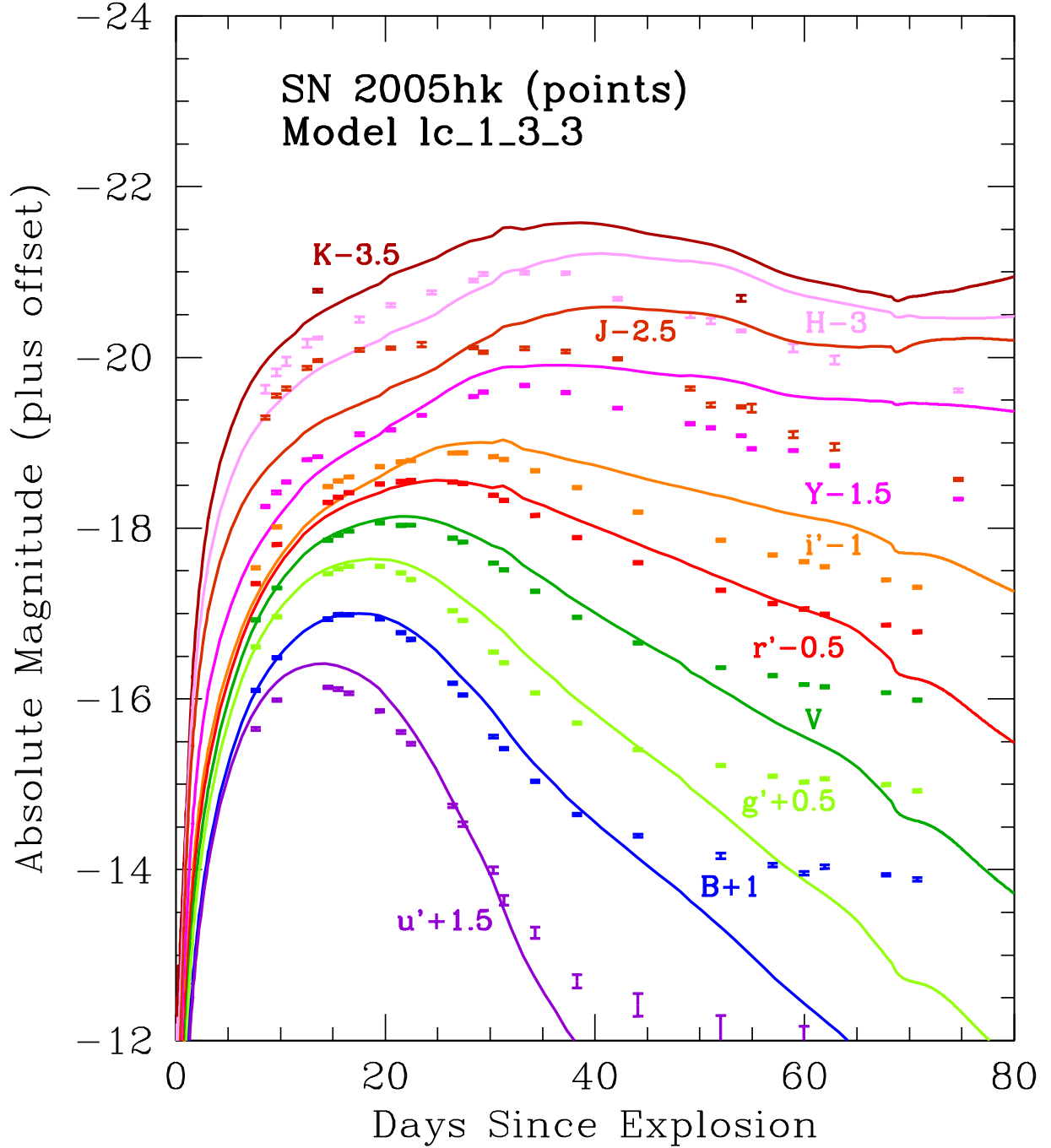
Fig. 16.— Comparison of calculations of the u'Bg'V'r'i' light curves for 3D deflagration model 1_3_3 with observations of SN 2005hk. The absolute magnitudes for SN 2005hk were calculated assuming a Galactic E(B - V)_{\text{Gal}} = 0.022 (Schlegel, Finkbeiner, & Davis 1998), a host galaxy reddening of E(B - V)_{\text{Host}} = 0.09 , and a Hubble constant of H_0 = 72 \text{ km s}^{-1} \text{ Mpc}^{-1} . The explosion is assumed to have occurred 17 days before B maximum.
